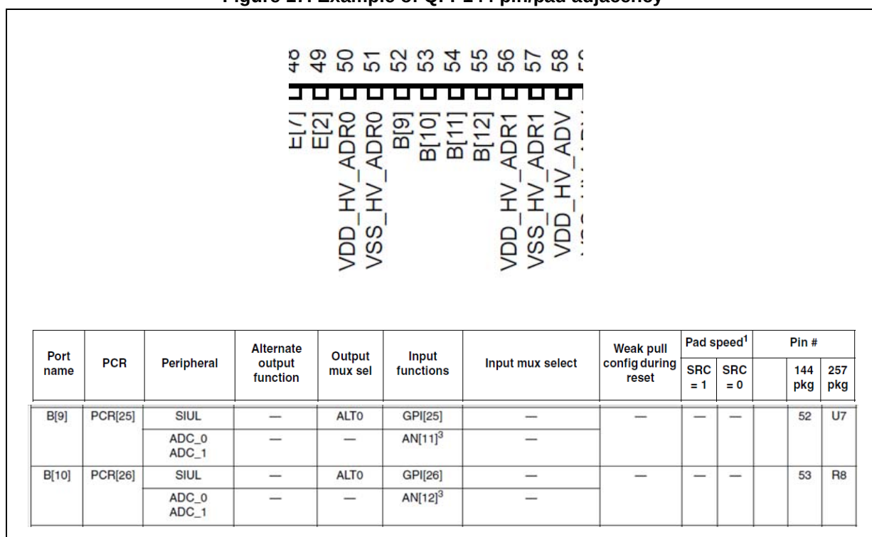
Figure 17. Example of QFP144 pin/pad adjacency
