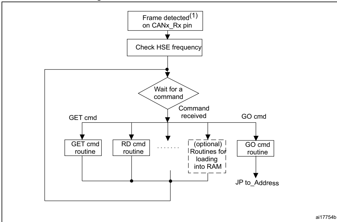
Figure 1. Bootloader for STM32 with CAN
