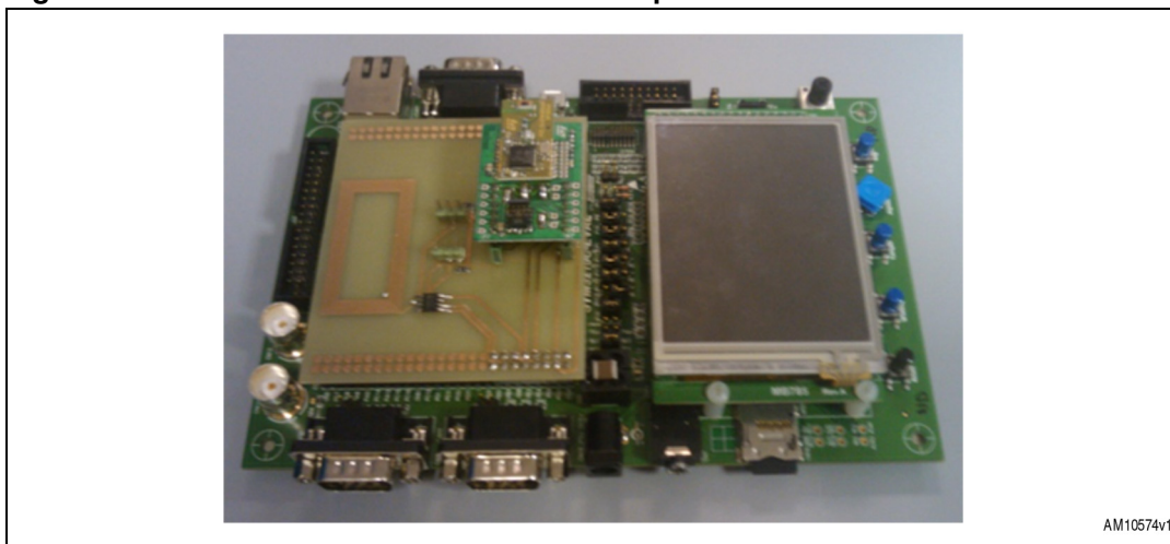
Figure 3. How to connect SPZB260-PRO adapter to the STM3210C-EVAL
