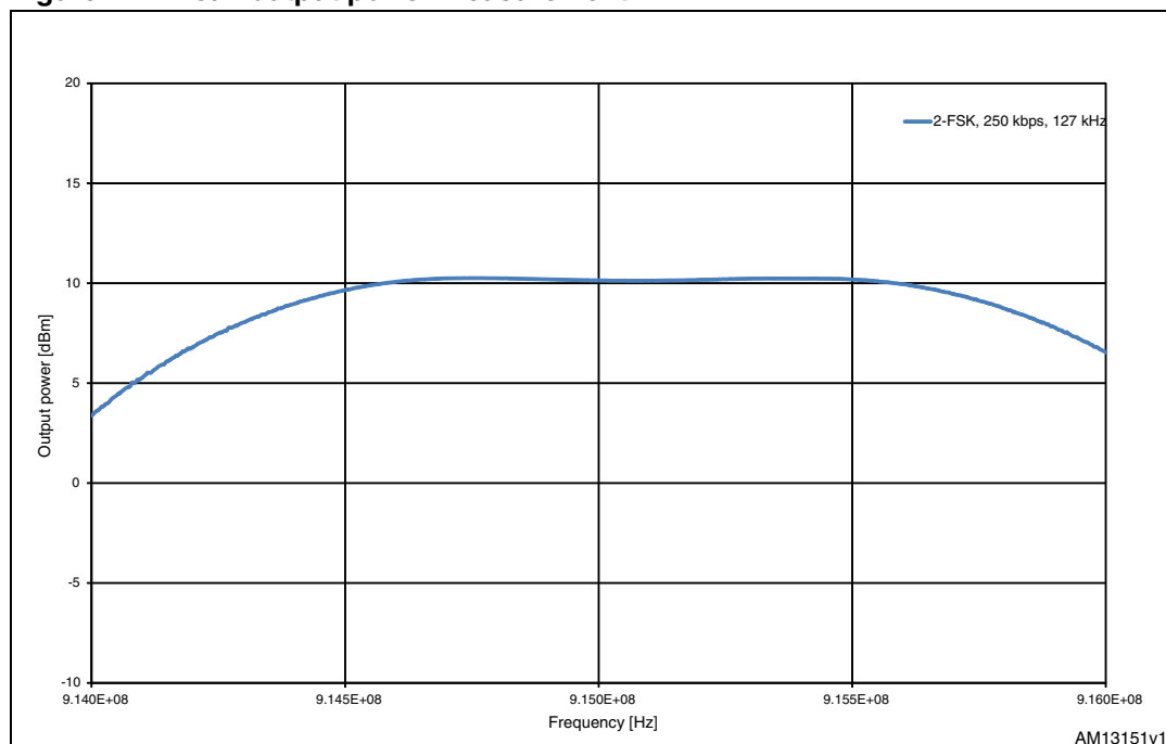
Figure 7. Peak output power measurement
