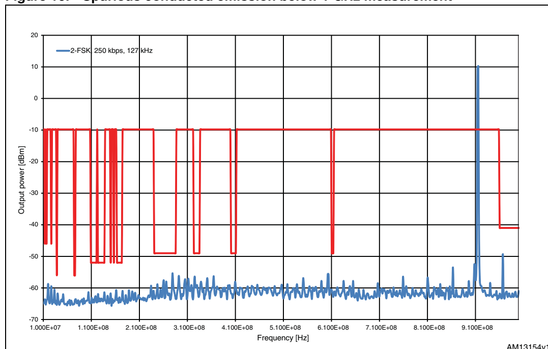
Figure 10. Spurious conducted emission below 1 GHz measurement
