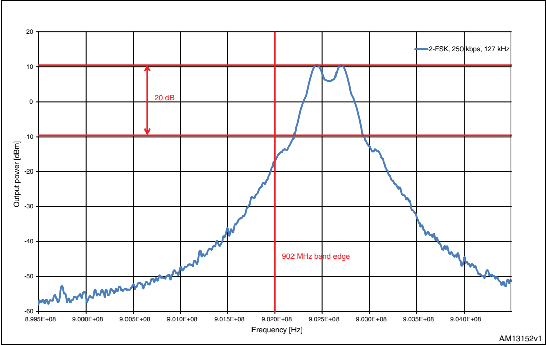
Figure 8. 902 MHz band edge conducted emission measurement
