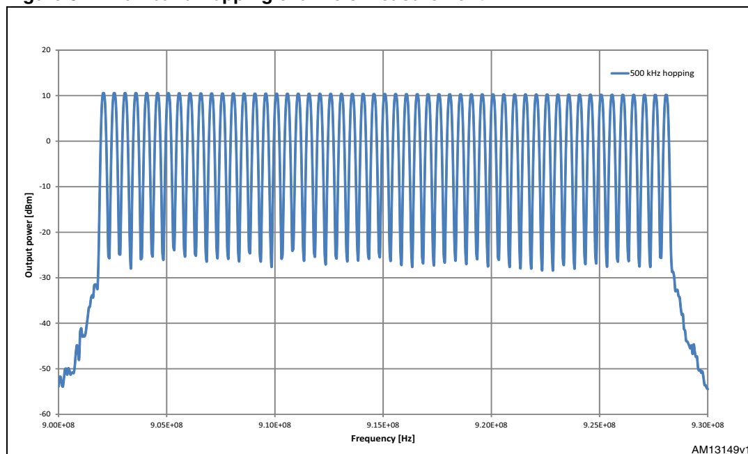
Figure 6. Full band hopping channels measurement
