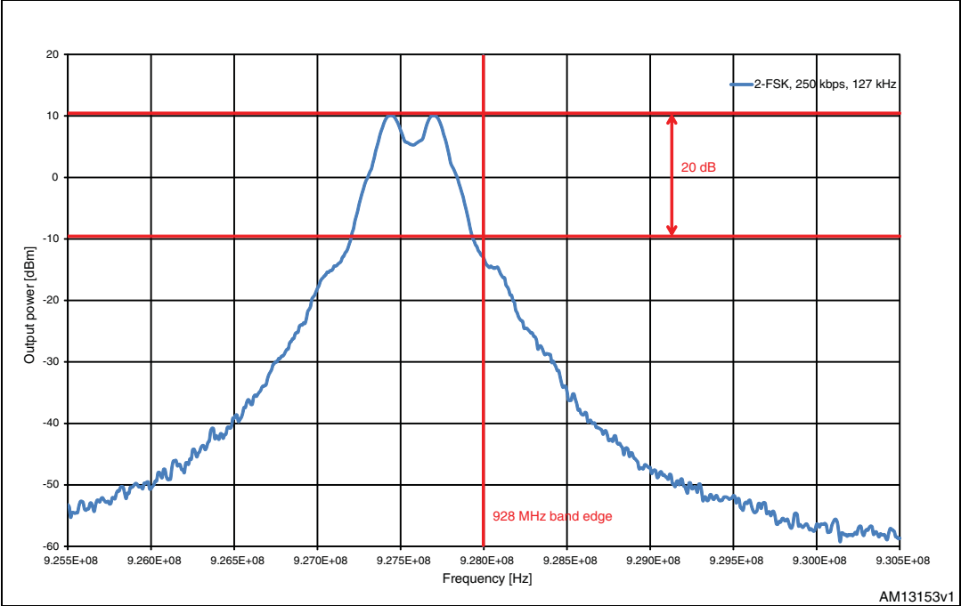
Figure 9. 928 MHz band edge conducted emission measurement
