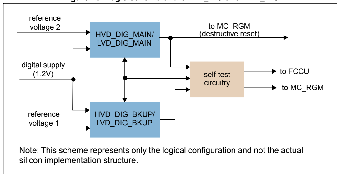
Figure 15. Logic scheme of the LVD_DIG and HVD_DIG
