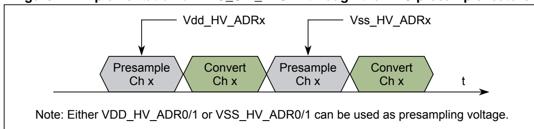
Figure 12. Implementation of ADC_SW_TEST2 through the ADC presample feature
