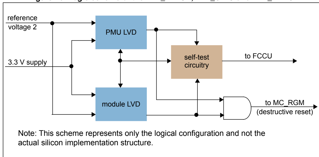
Figure 16. Logic scheme of the LVD_FLASH, LVD_GPIO and LVD_VREG
