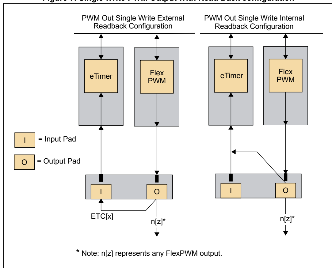
Figure 7. Single Write PWM Output With Read Back configuration
