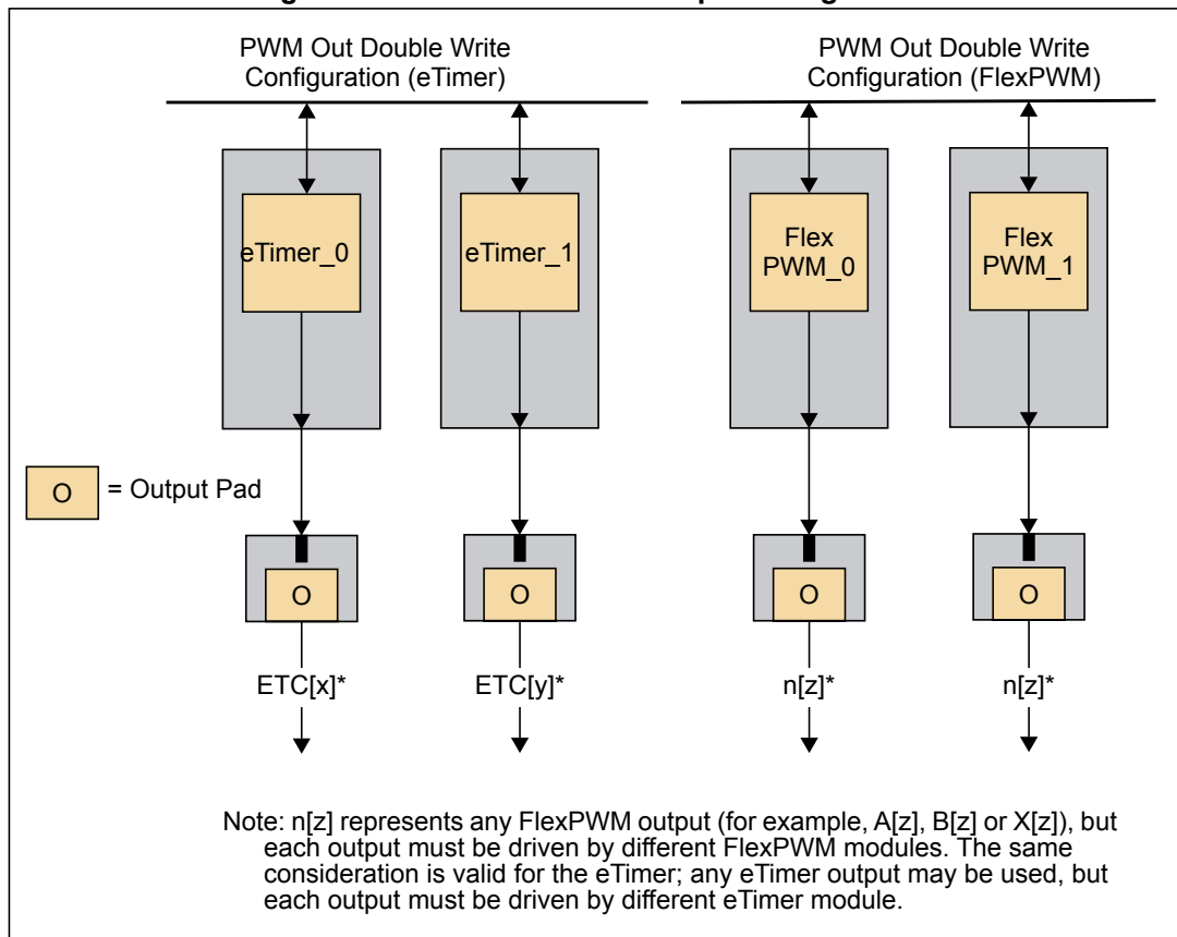
Figure 6. Double Write PWM Output configuration
