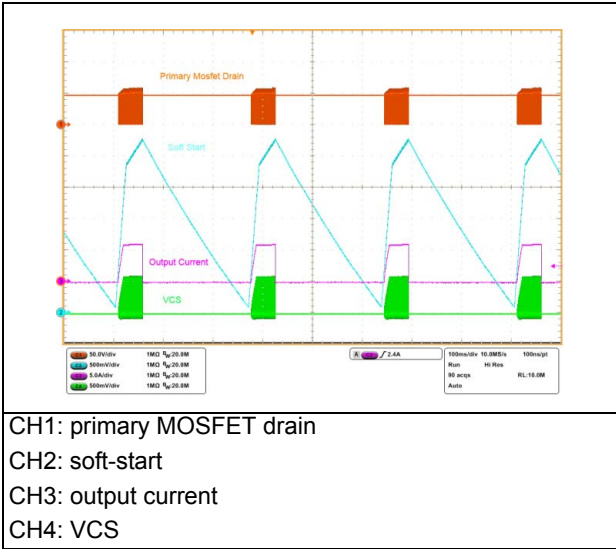
Figure 22. OCP steady state - full load
