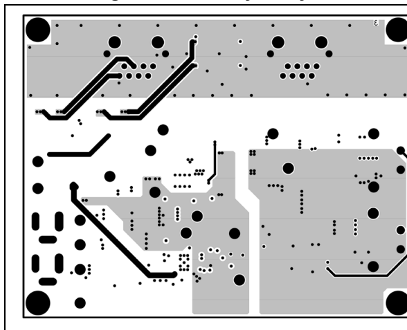
Figure 33. PCB layer: layer 3
