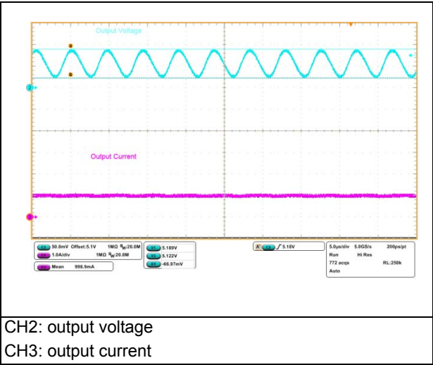
Figure 8. Ripple 5 V at 1 A removing L4 filter
