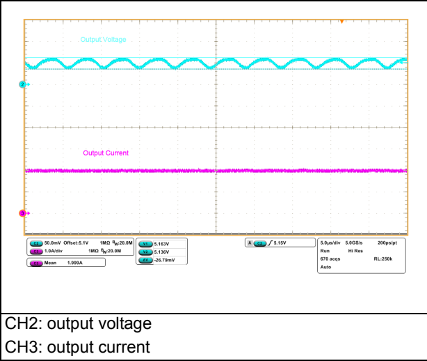
Figure 5. Ripple 5 V at 2 A
