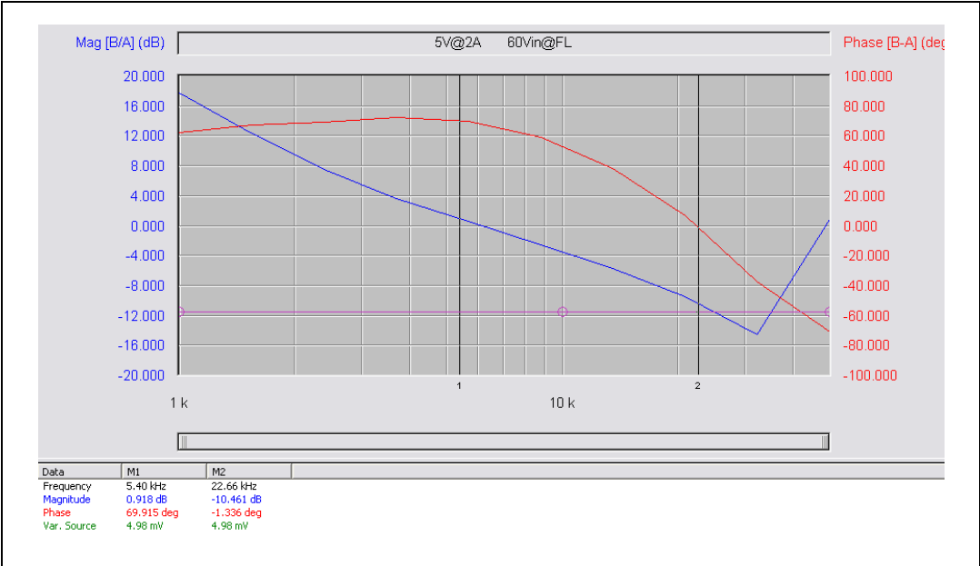
Figure 29. Gain loop full load 60 V
