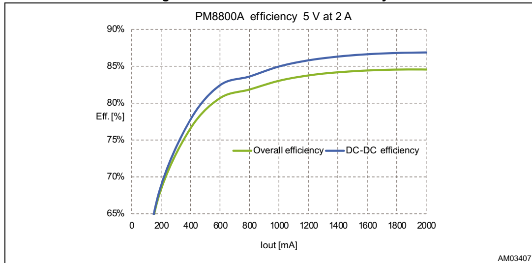
Figure 3. Overall and DC/DC efficiency
