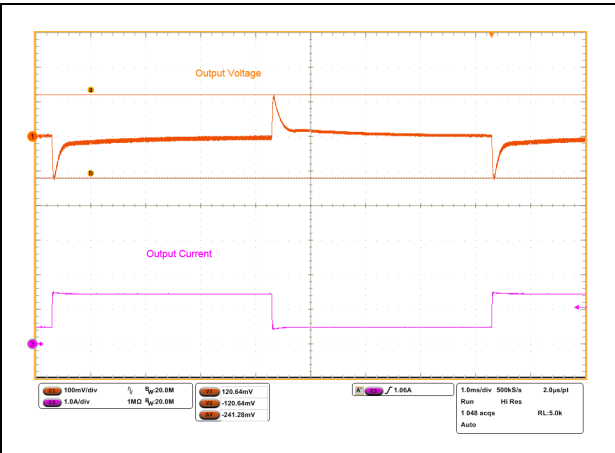
Figure 19. Dynamic load 750 mA - 250 mA
