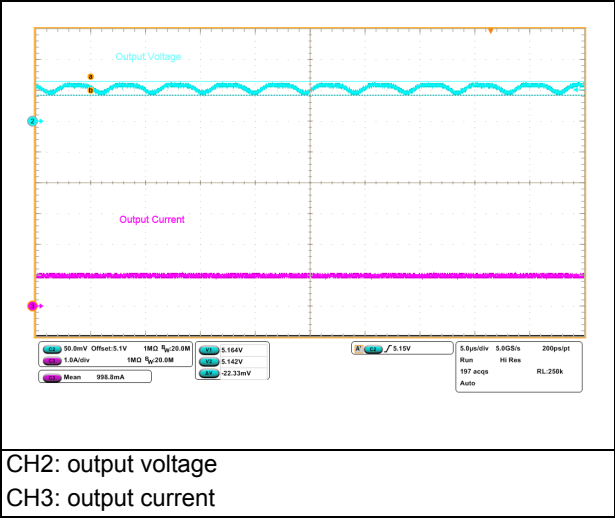
Figure 6. Ripple 5 V at 1 A
