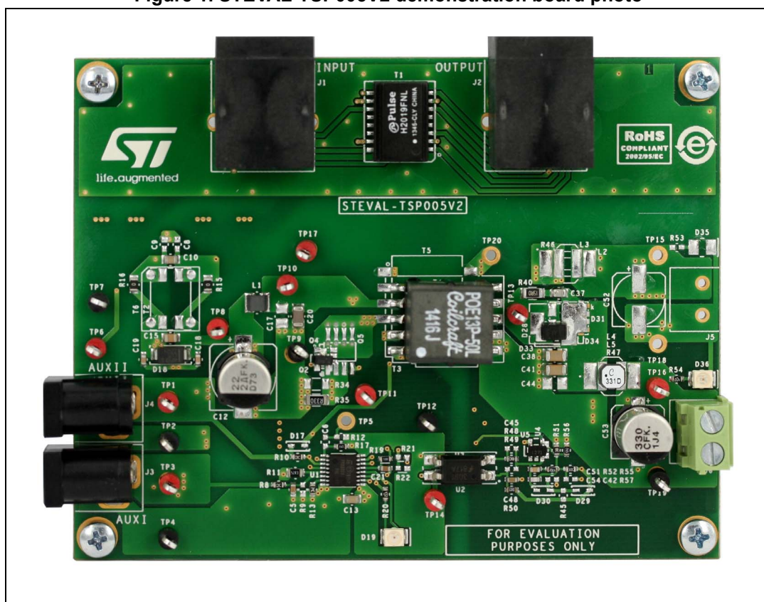
Figure 1. STEVAL-TSP005V2 demonstration board photo
