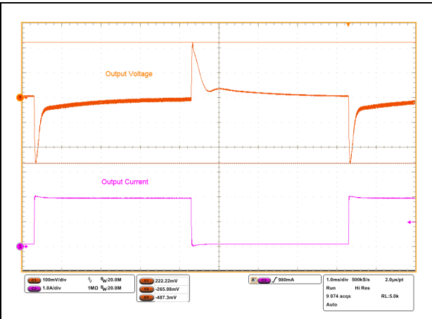
Figure 18. Dynamic load 2 A - 200 mA
