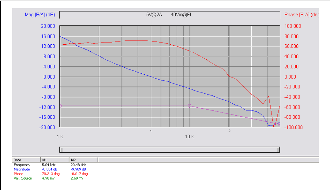
Figure 28. Gain loop full load 40 V
