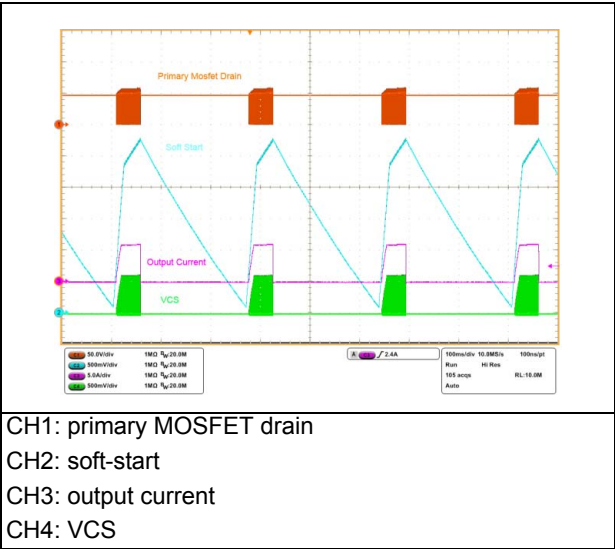
Figure 23. OCP steady state- no load
