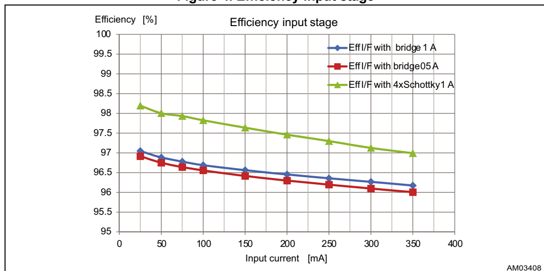
Figure 4. Efficiency input stage
