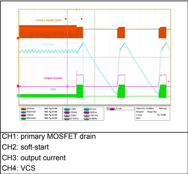
Figure 23. OCP steady state- no load
