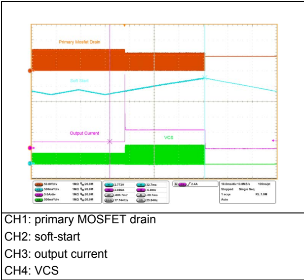
Figure 22. OCP steady state - full load
