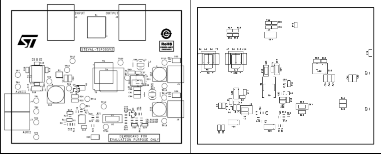
Figure 35. PCB Layer: components on top side Figure 36. PCB Layer: components on bottom side
