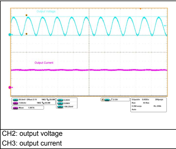
Figure 7. Ripple 5 V at 2 A removing L4 filter
