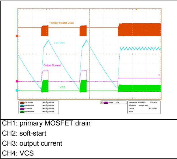
Figure 24. OCP removed - full load
