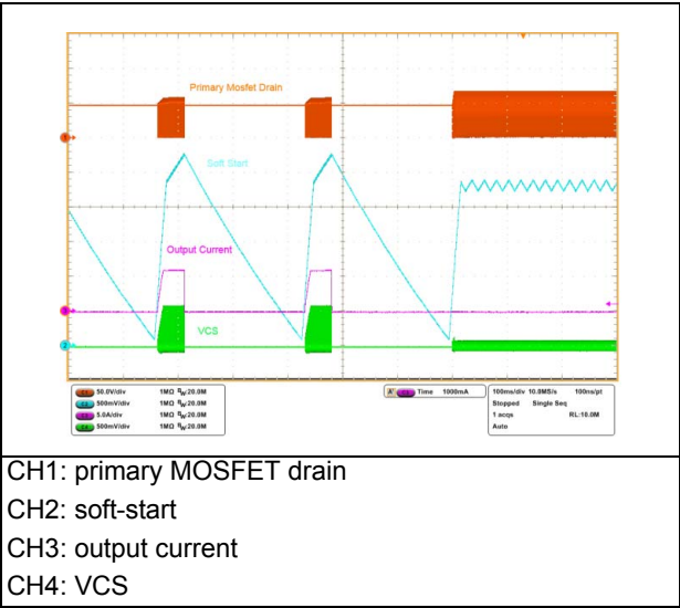
Figure 25. OCP removed - no load
