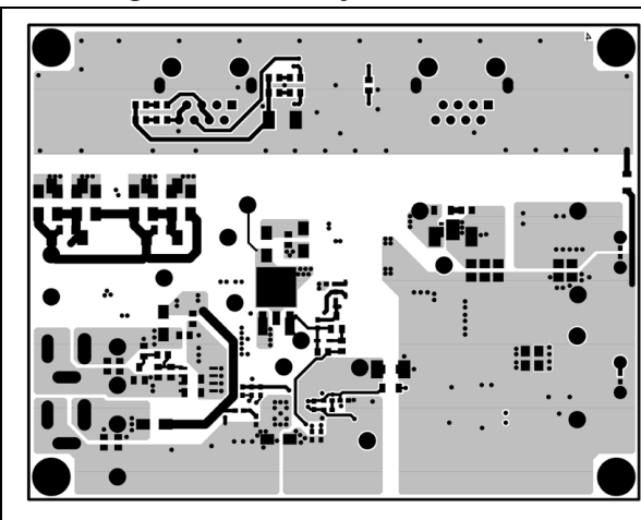
Figure 34. PCB layer: bottom view
