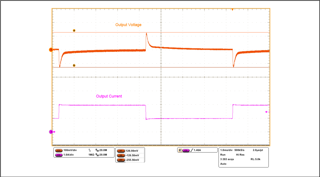
Figure 18. Dynamic load 2 A - 200 mA
