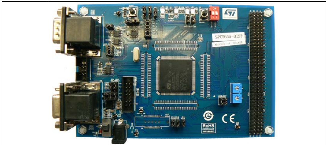
Figure 1. SPC564A-DISP Discovery Plus board with SPC564A70L7
