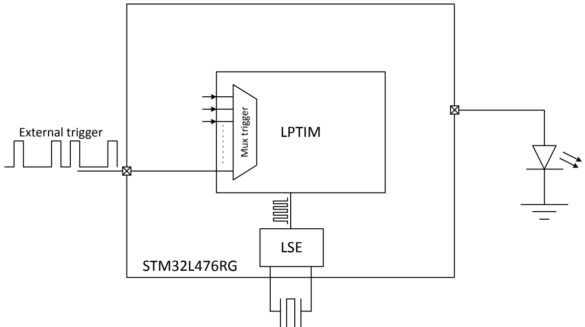
Figure 9. Timeout wakeup mode architecture
