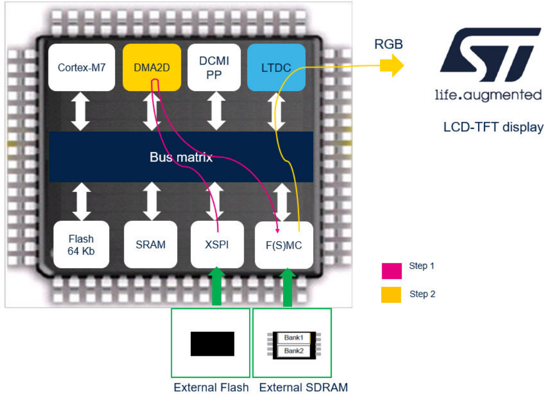
Figure 2. STM32H7R7/7S7 display application use case
