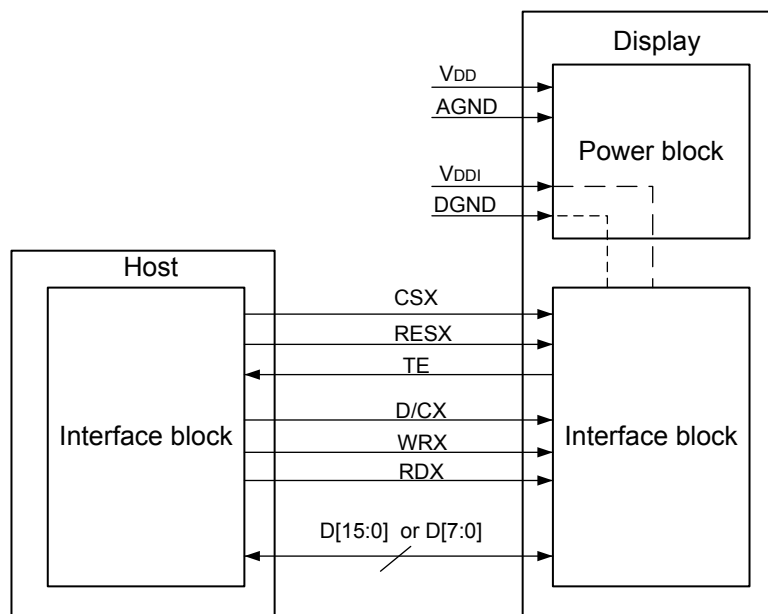
Figure 3. Display bus interface specification
