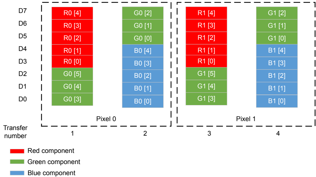
Figure 7. 16 bpp over 8-bit interface color coding
