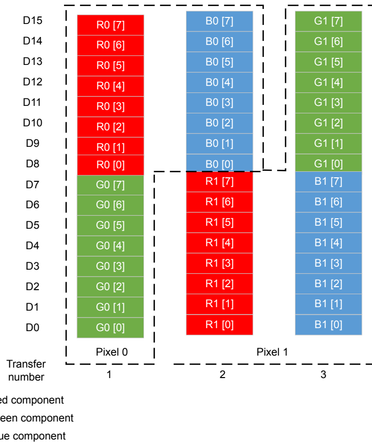
Figure 6. 24 bpp over 16-bit interface color coding
