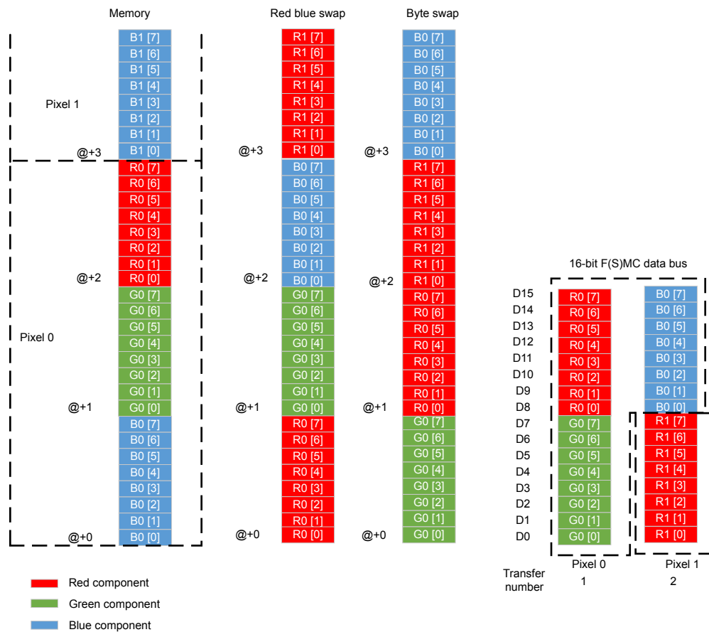
Figure 9. DMA2D operations to support 24 bpp over 16-bit interface
