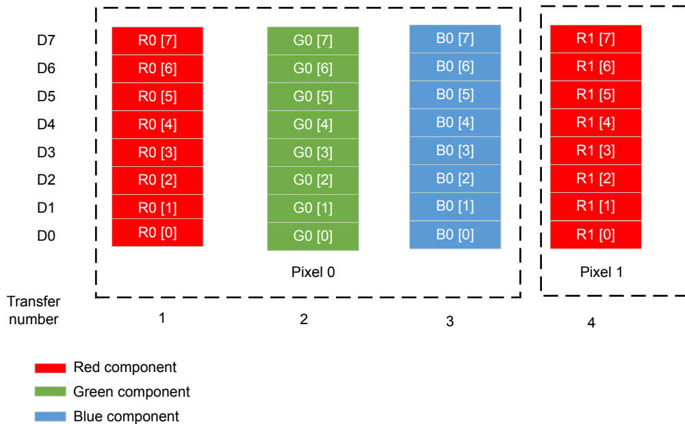
Figure 8. 24 bpp over 8-bit interface color coding
