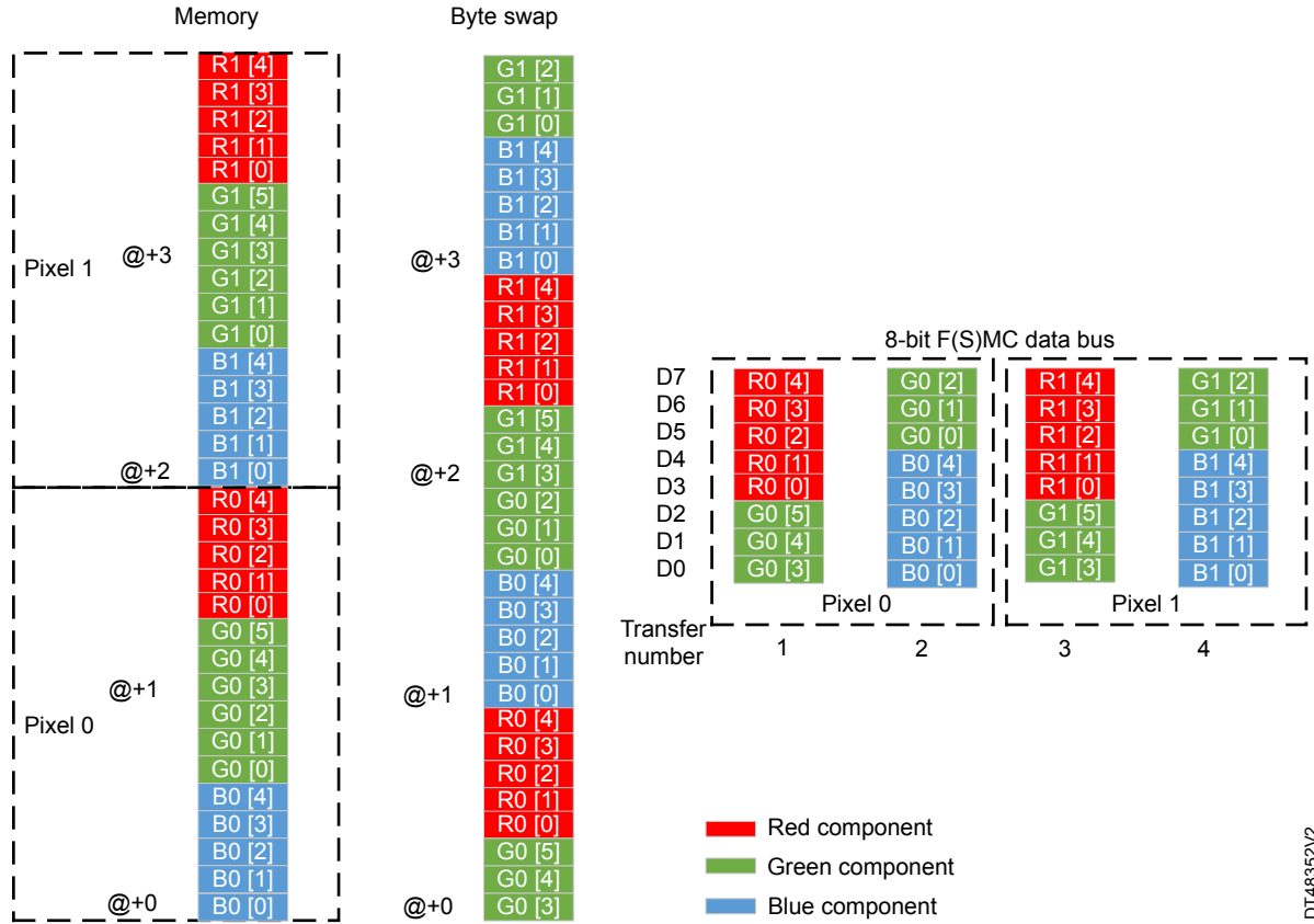
Figure 11. DMA2D operations to support 16 bpp over 8-bit interface
