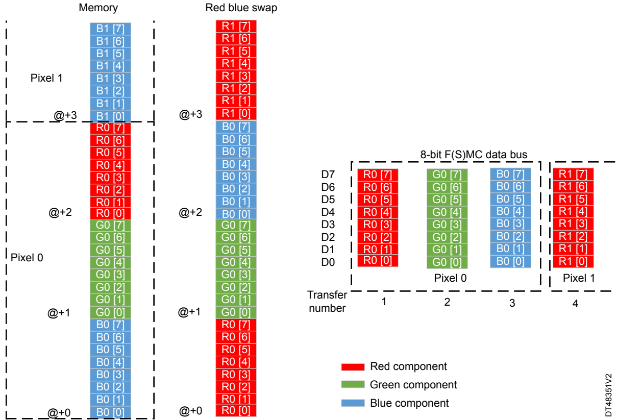
Figure 10. DMA2D operations to support 24 bpp over 8-bit interface
