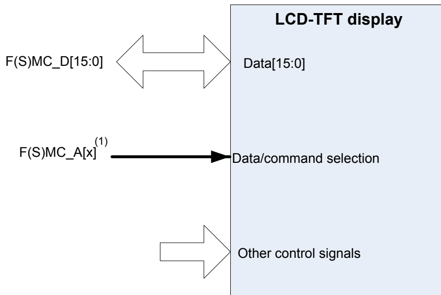
Figure 5. Automatic control of LCD-TFT display data/command by F(S)MC interface
