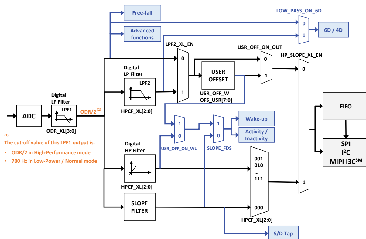
Figure 2. Accelerometer filtering chain (UI path)
