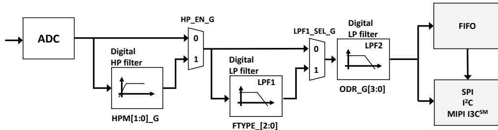
Figure 4. Gyroscope digital chain - mode 1 and mode 2
