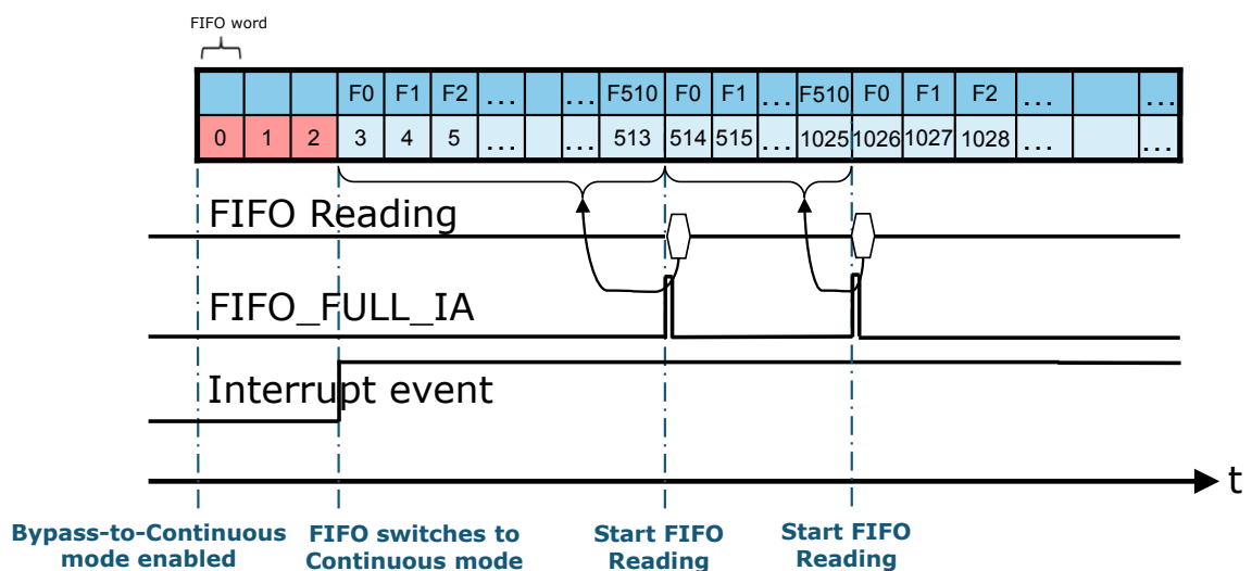
Figure 31. Bypass-to-continuous mode
