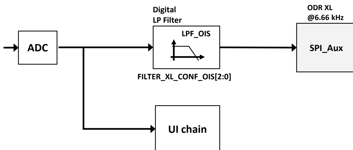
Figure 26. Accelerometer filtering chain (mode 4)
