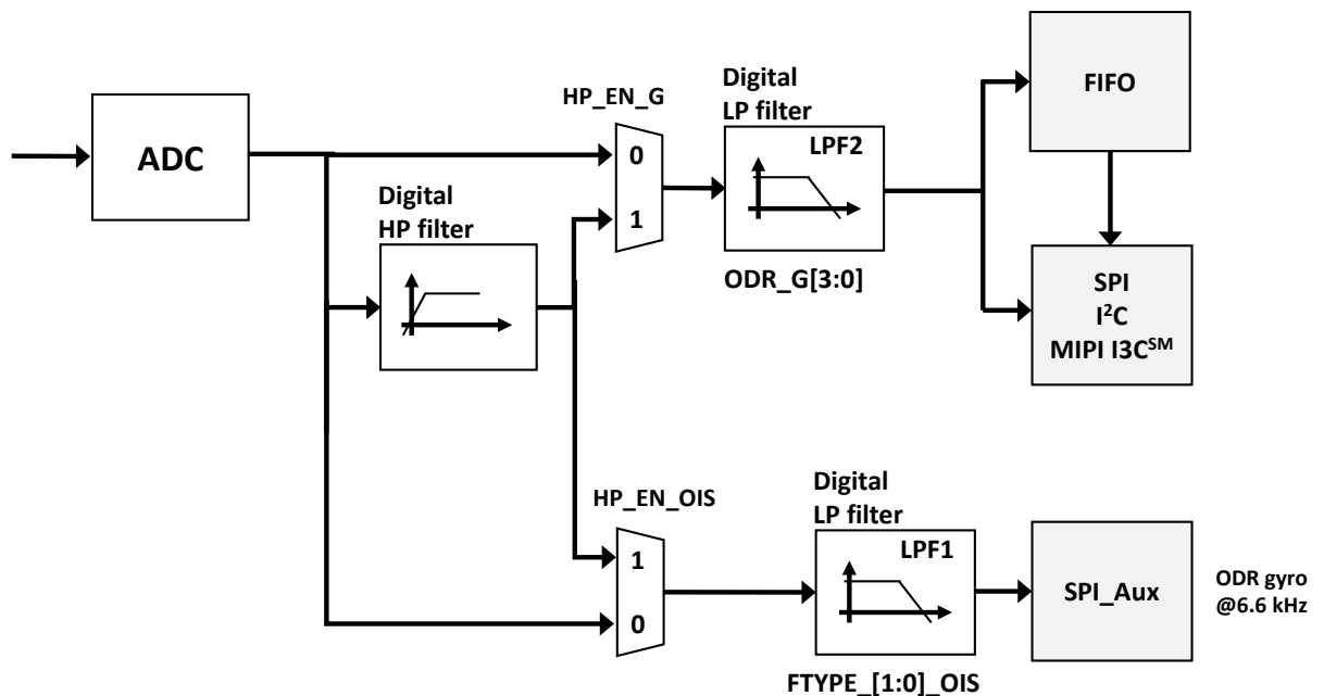
Figure 5. Gyroscope digital chain - mode 3 and mode 4
