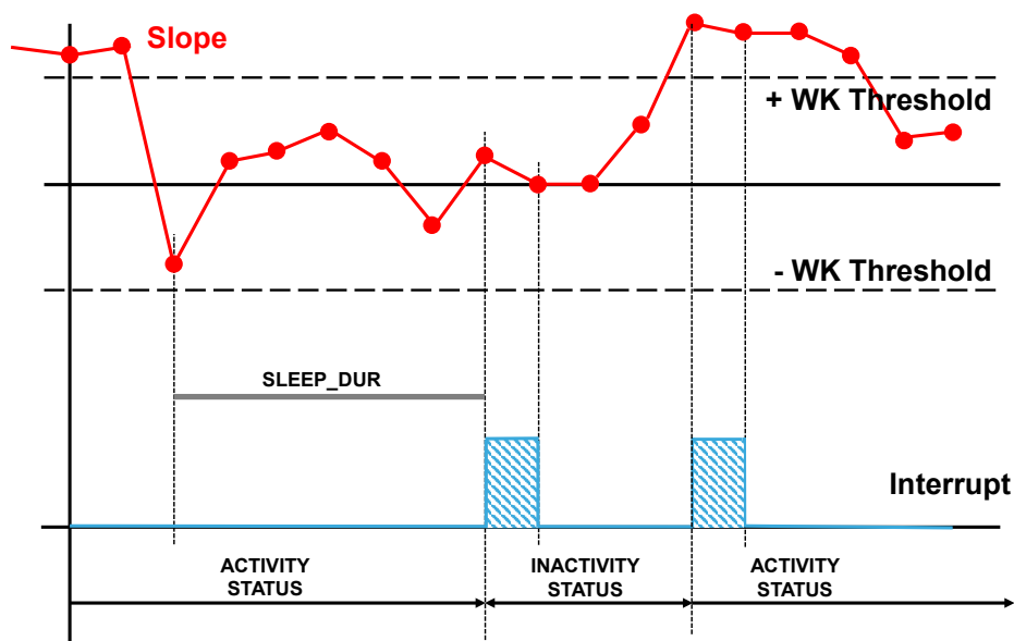
Figure 19. Activity/Inactivity recognition (using the slope filter)
