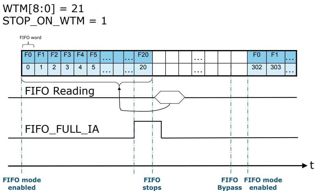
Figure 34. FIFO threshold (STOP_ON_WTM = 1) in FIFO mode
