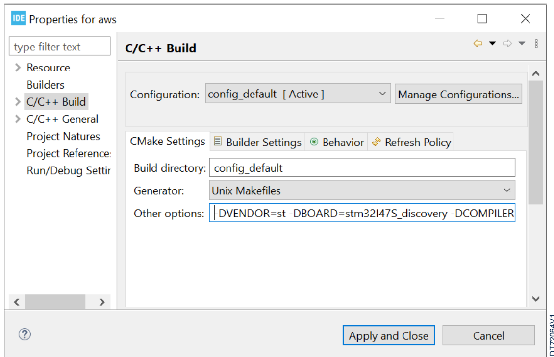
Figure 11. CMake build options
