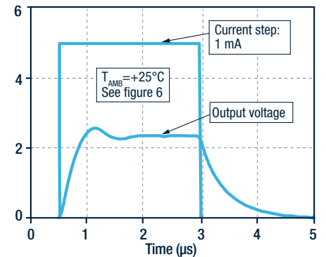
Pulse response for I_k = 1 mA
