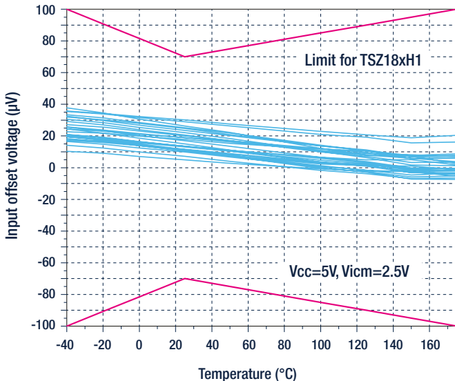
Input offset voltage vs temperature
