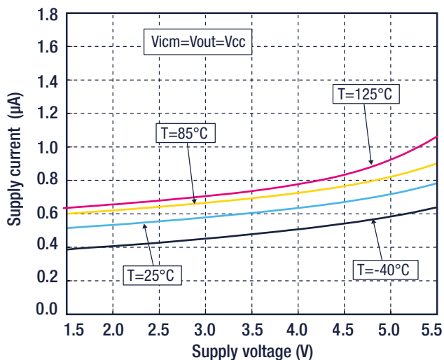
Supply current vs. supply voltage at high VICM
