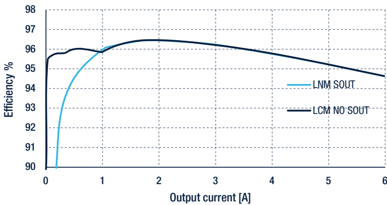
Efficiency curves V IN = 5 V, V OUT = 3.3 V, f sw = 2.25 MHz
