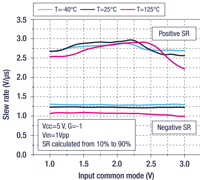
Slew rate vs. input common mode voltage at V_{cc}=5 V
