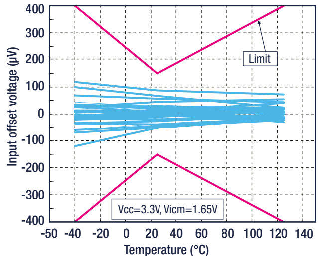
Input offset voltage vs. temperature at 3.3V
