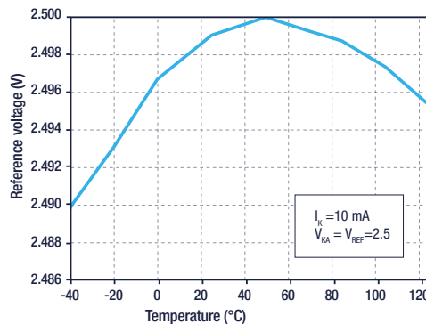
Reference voltage vs. temperature
