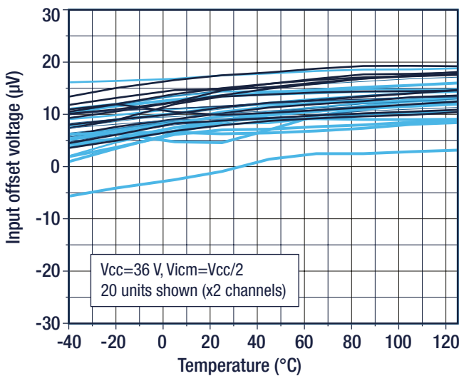
Input offset voltage vs. temperature for V_{cc} = 36 V
