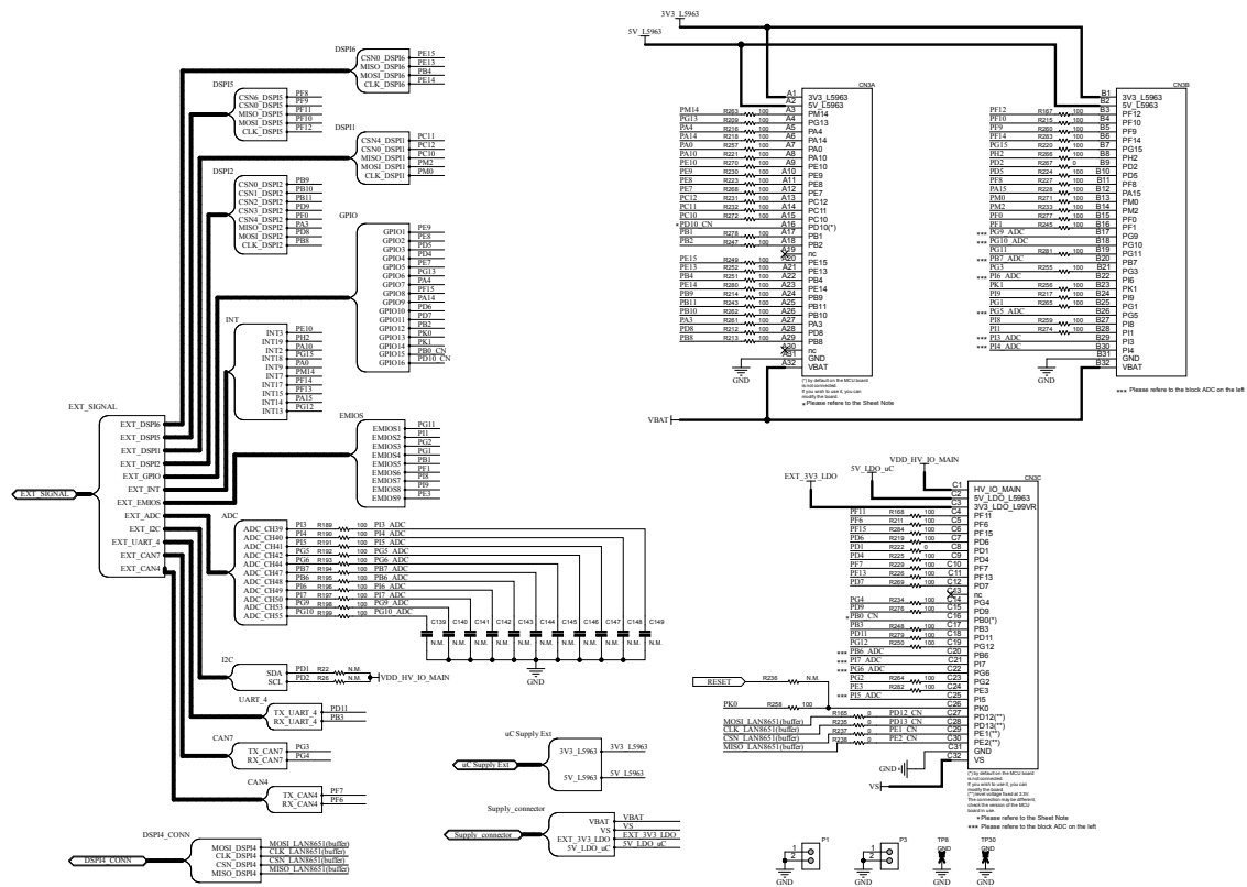
Figure 13. AEK-MCU-C4M2 circuit schematic (10 of 11)
