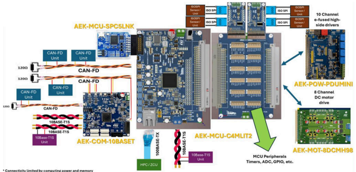
Figure 3. Automotive edge node block diagram
