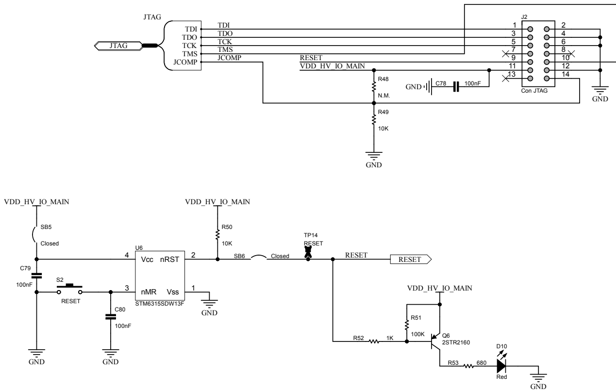
Figure 8. AEK-MCU-C4M2 circuit schematic (5 of 11)
