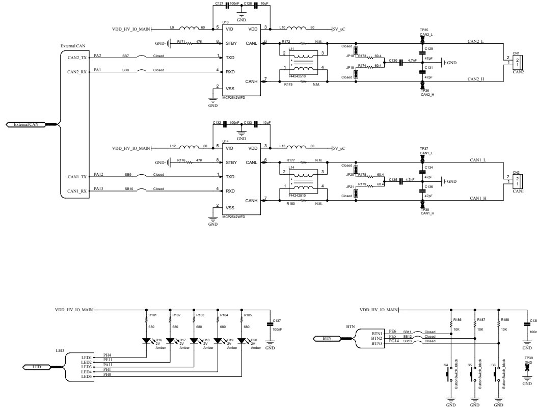
Figure 12. AEK-MCU-C4M2 circuit schematic (9 of 11)
