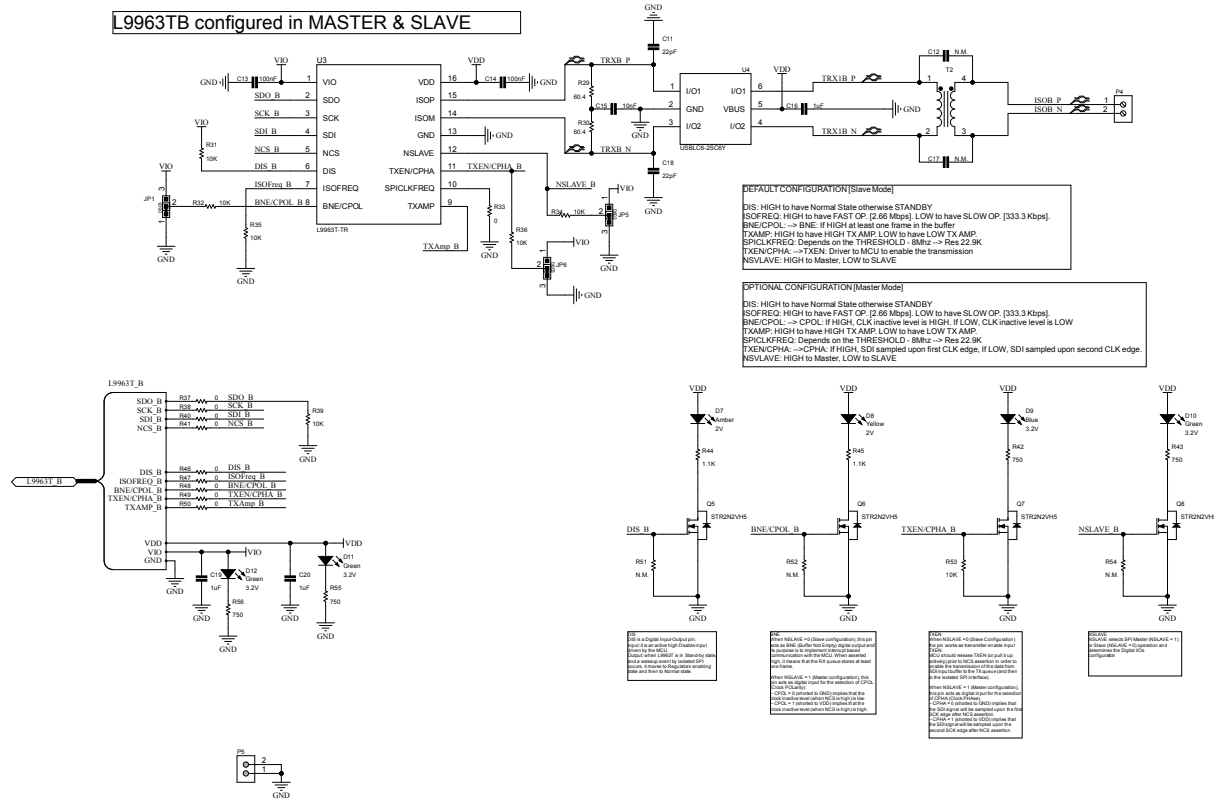
Figure 16. AEK-CON-LTA2 circuit schematic (1 of 3)
