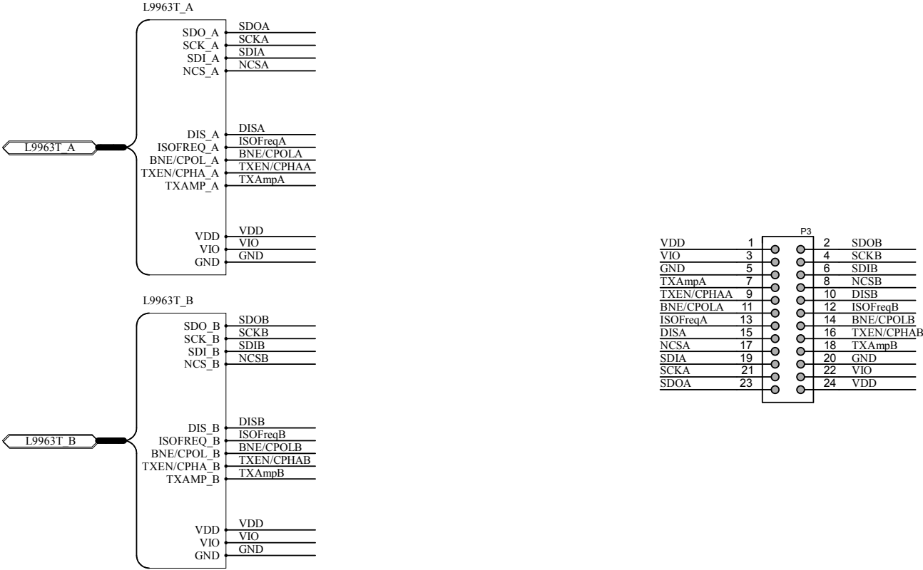
Figure 18. AEK-CON-LTA2 circuit schematic (3 of 3)
