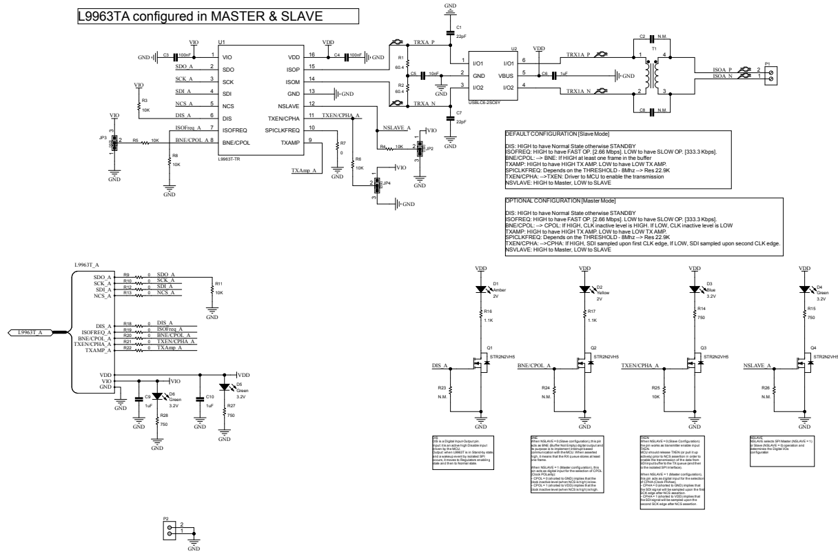
Figure 17. AEK-CON-LTA2 circuit schematic (2 of 3)
