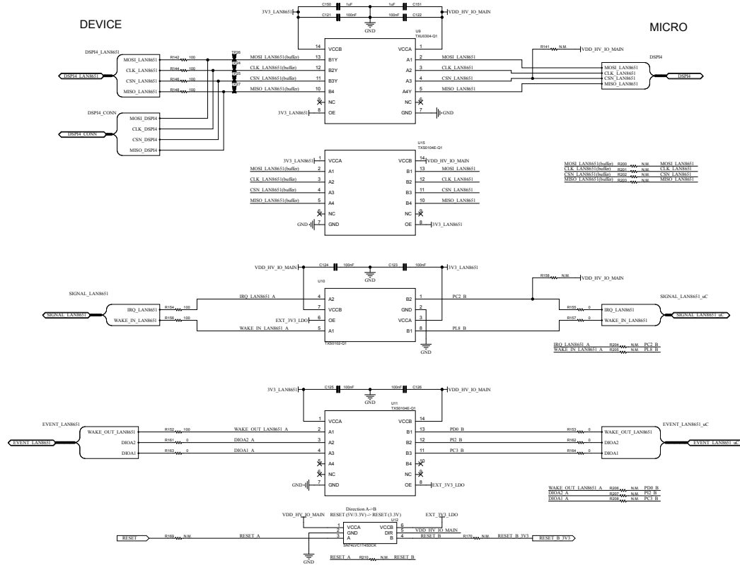
Figure 11. AEK-MCU-C4M2 circuit schematic (8 of 11)
