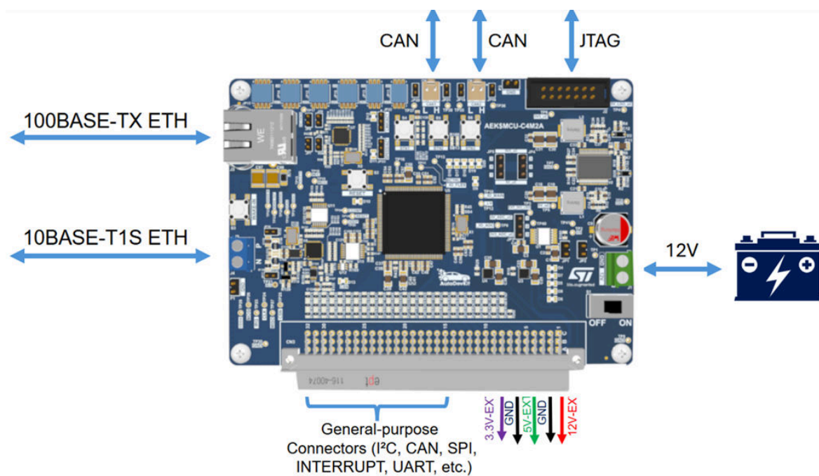
Figure 2. AEK-MCU-C4M2 connection diagram
