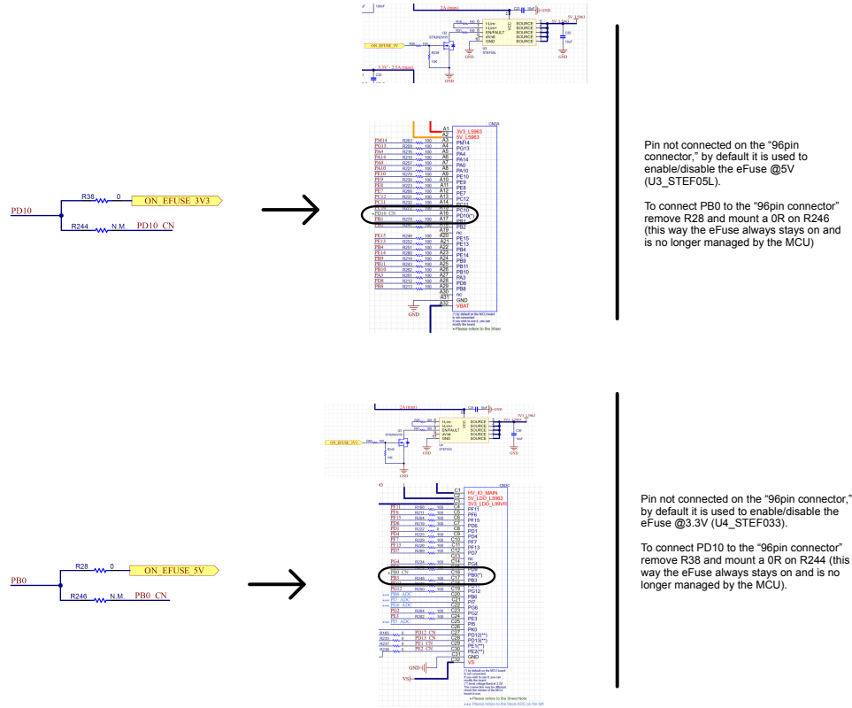
Figure 14. AEK-MCU-C4M2 circuit schematic (11 of 11)
