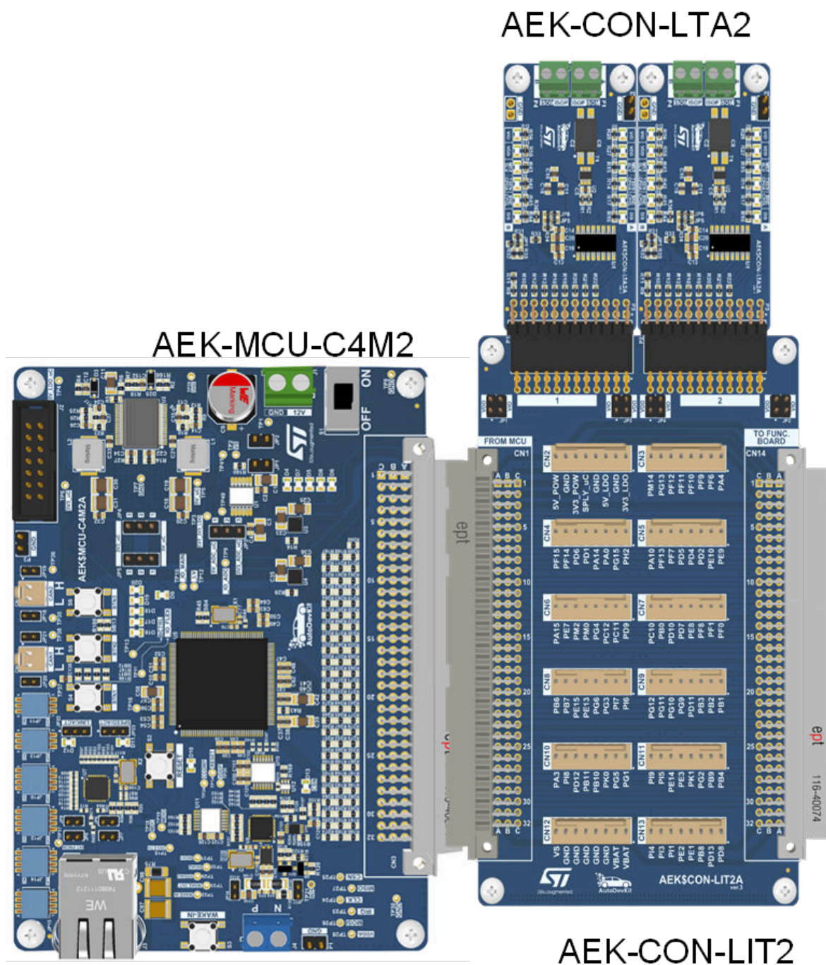
Figure 1. AEK-MCU-C4MLIT2 evaluation kit connections
