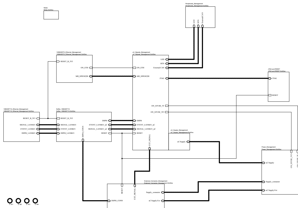
Figure 4. AEK-MCU-C4M2 circuit schematic (1 of 11)
