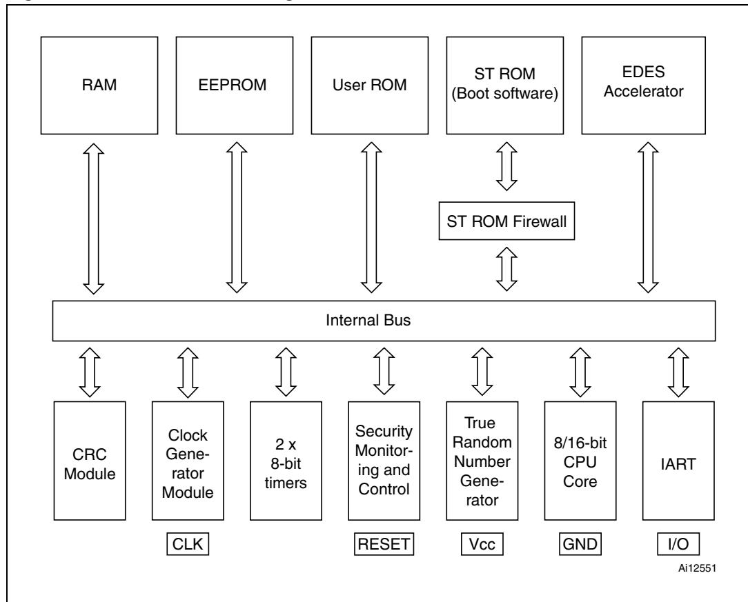
Figure 1. ST23YS08 block diagram
