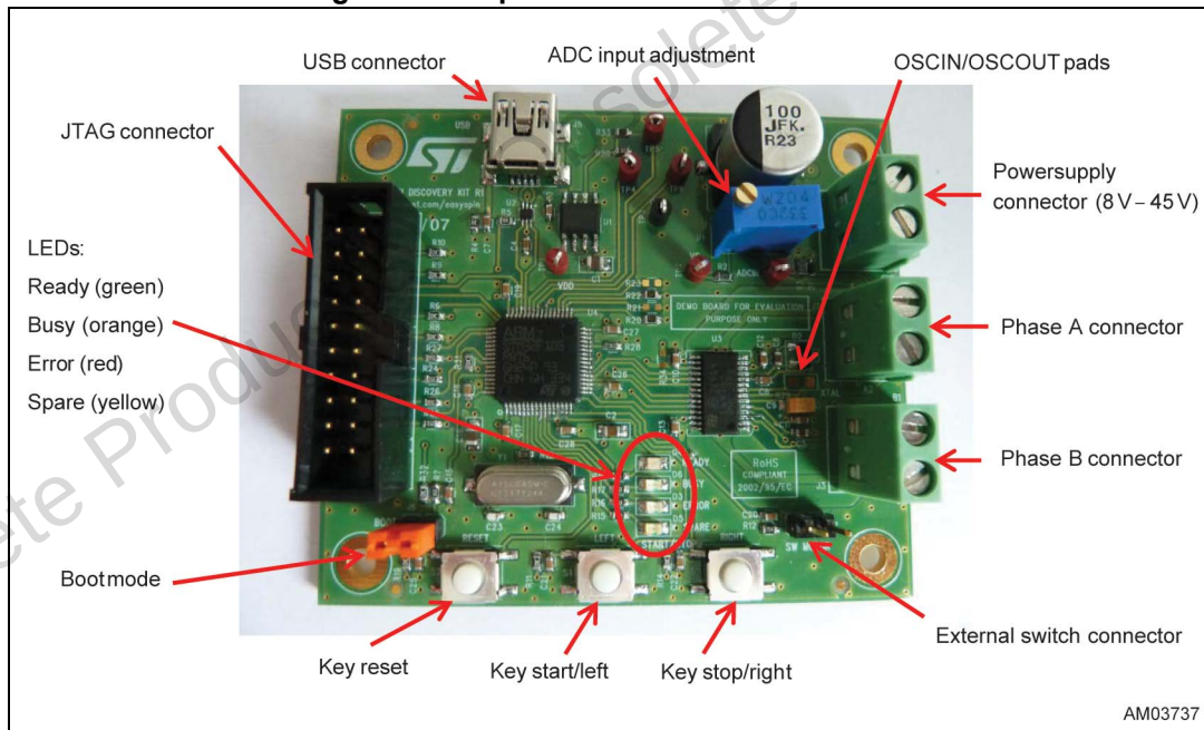
Figure 1. Jumpers and connectors location
