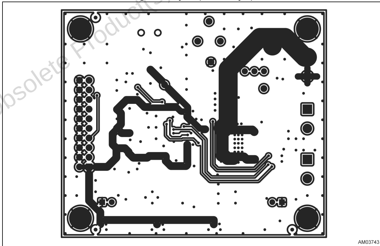
Figure 6. Layout (bottom layer) of the EVAL6474H-DISC board.
