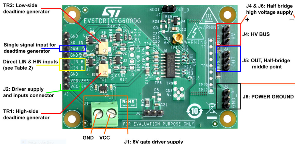
Figure 3. EVSTDRIVE600DG - Supply and signal connection
