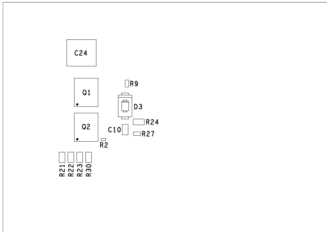
Figure 5. EVSTDRIVEG600DG - Layout (component placement bottom view)
