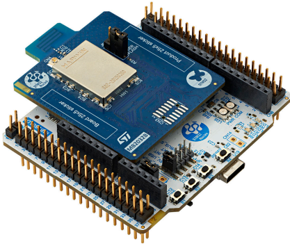
NUCLEO-WB09KE global view. Picture is not contractual.
