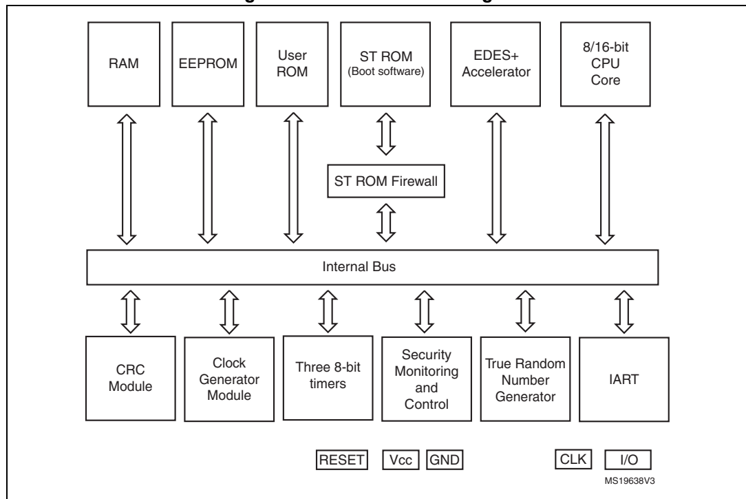
Figure 1. SB23Z012 block diagram
