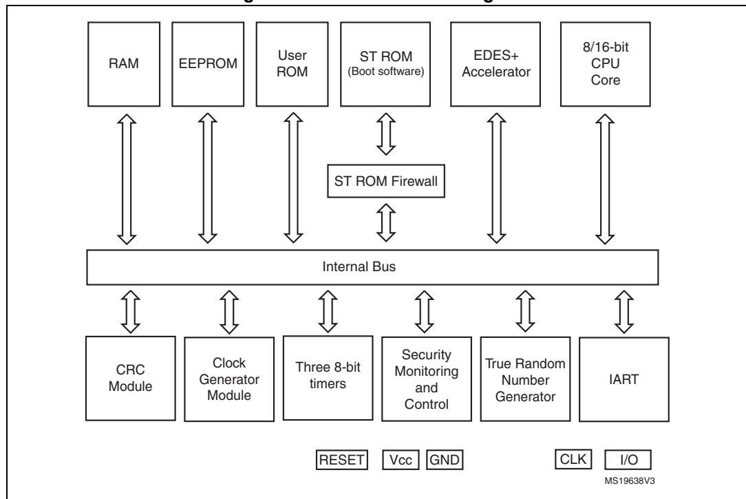
Figure 1. SB23ZE04 block diagram
