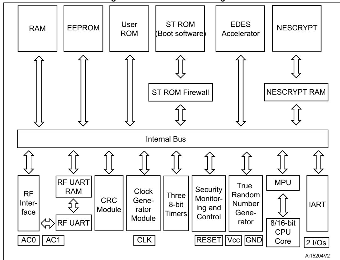
Figure 1. ST23YR48 block diagram
