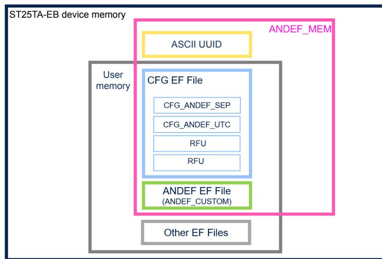
Figure 6. ANDEF_MEM content
