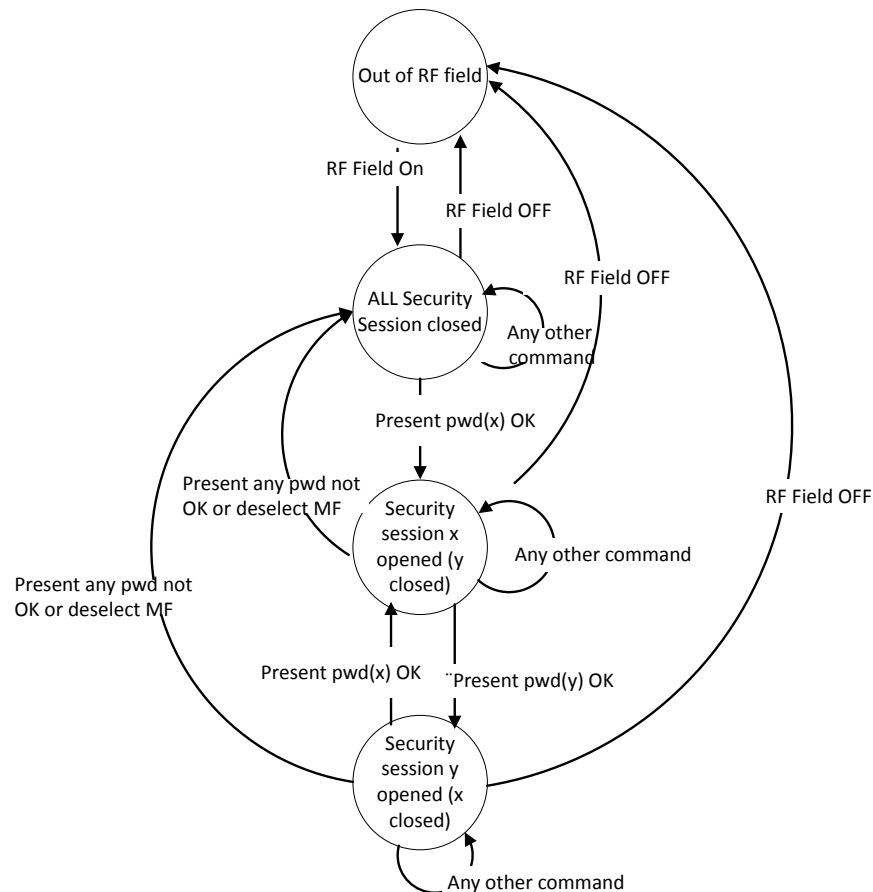
Figure 4. ST25TA-EB security session management
