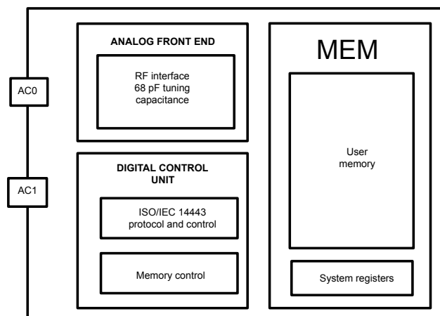
Figure 1. ST25TA-EB block diagram
