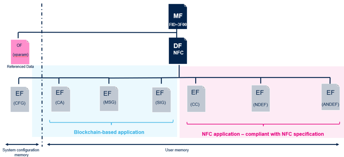
Figure 3. ST25TA-EB file system organization
