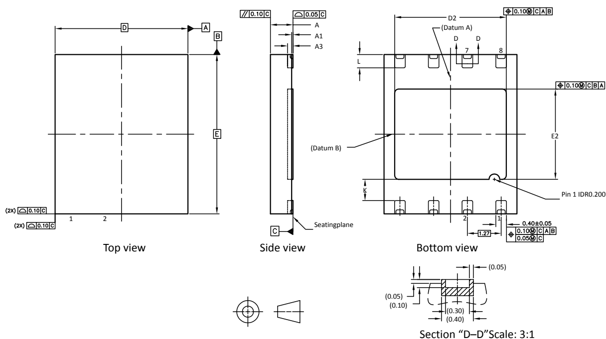
Figure 4. VFDFPN8 - outline
