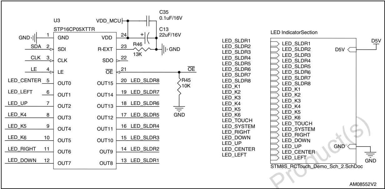
Figure 2. LED indicator
