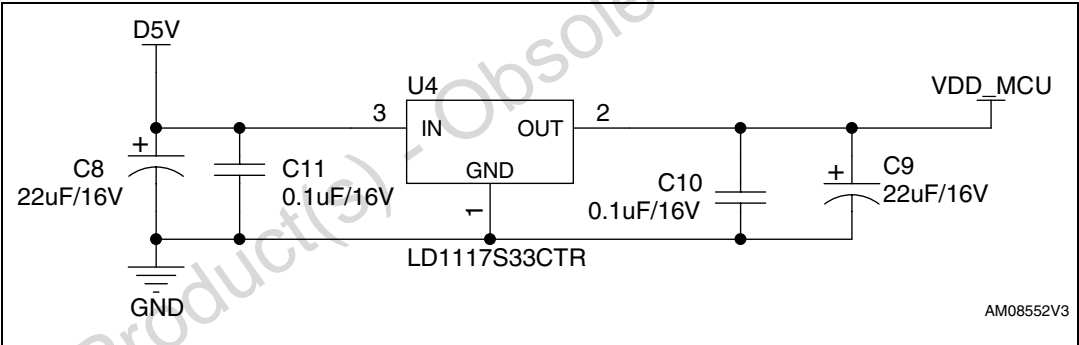
Figure 3. Power supply
