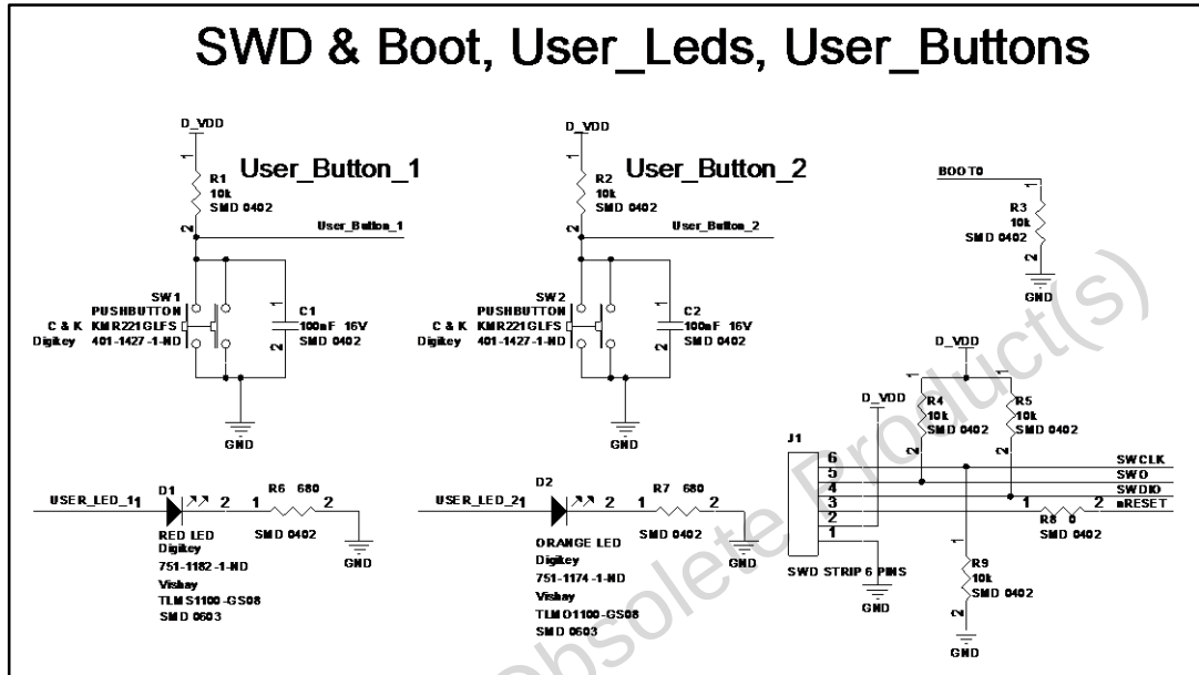
Figure 1: STEVAL-IDS001V5M part 1
