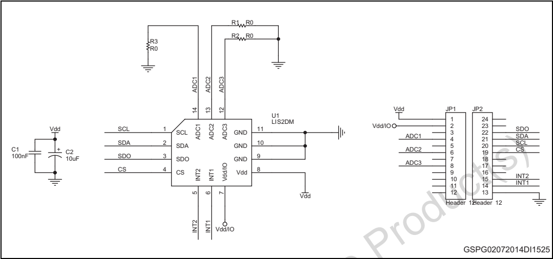
Figure 1. STEVAL-MKI152V1 circuit schematic
