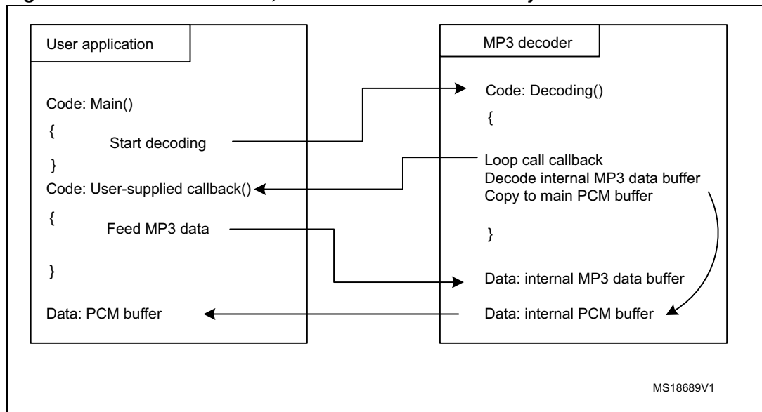
Figure 1. MP3 decoder flow, in “Pull” mode: callback way
