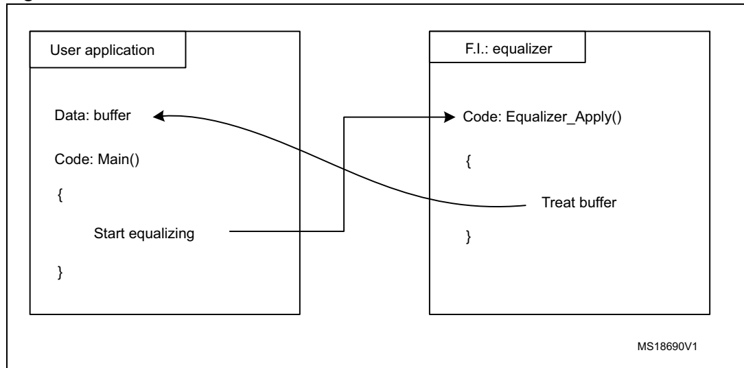
Figure 2. “Push” mode: no callback
