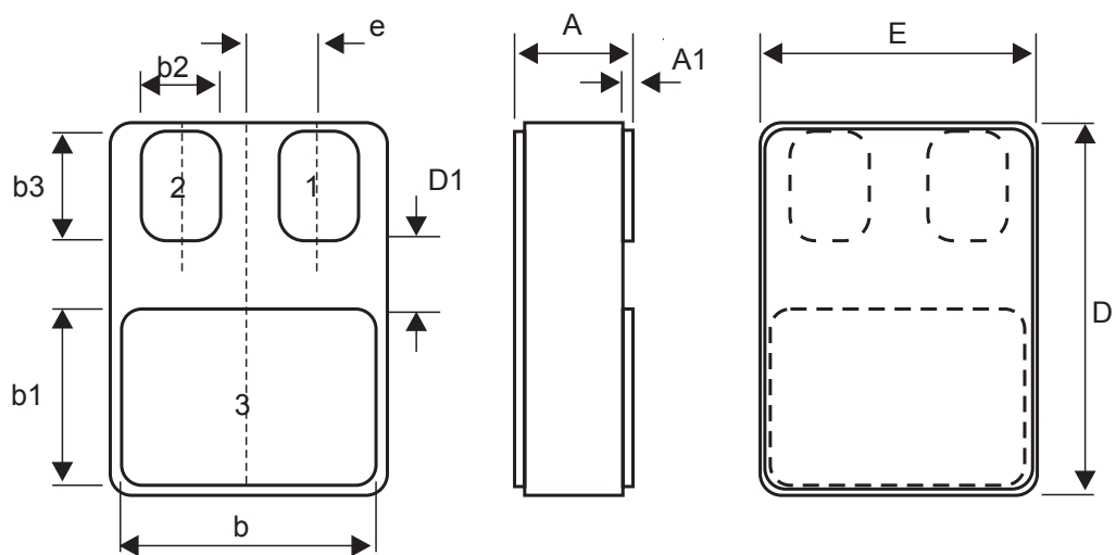
Figure 1. Surface mount SMD.5 package outline (3-terminal)
