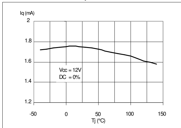
Figure 7. Quiescent current vs junction temperature
