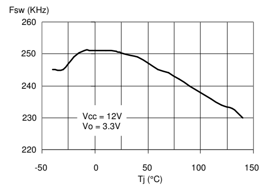
Figure 6. Switching frequency vs junction temperature
