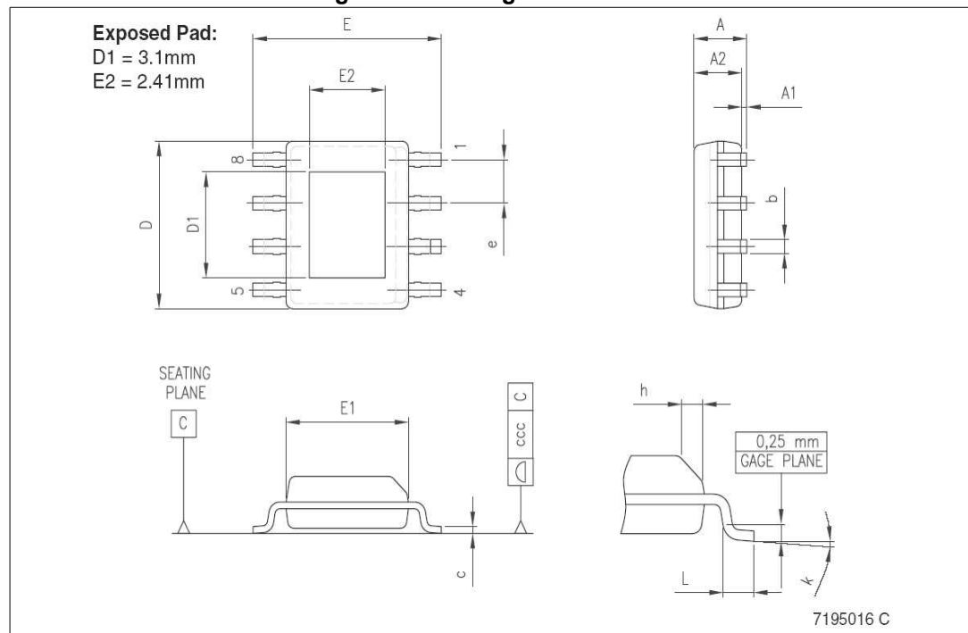
Figure 20. Package dimensions
