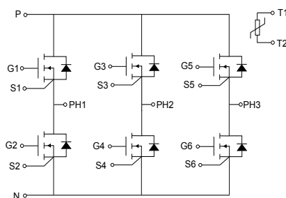
ACEPACK DMT-32 zig-zag
