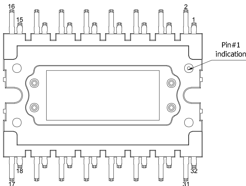
Figure 1. ACEPACK DMT-32 zig-zag pin layout (bottom view)
