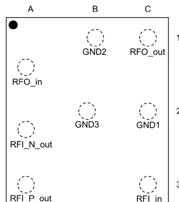
Figure 10. Top view
