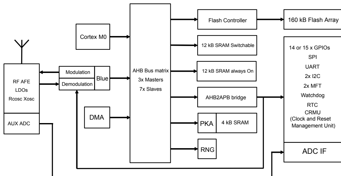
Figure 1. BlueNRG-1 architecture
