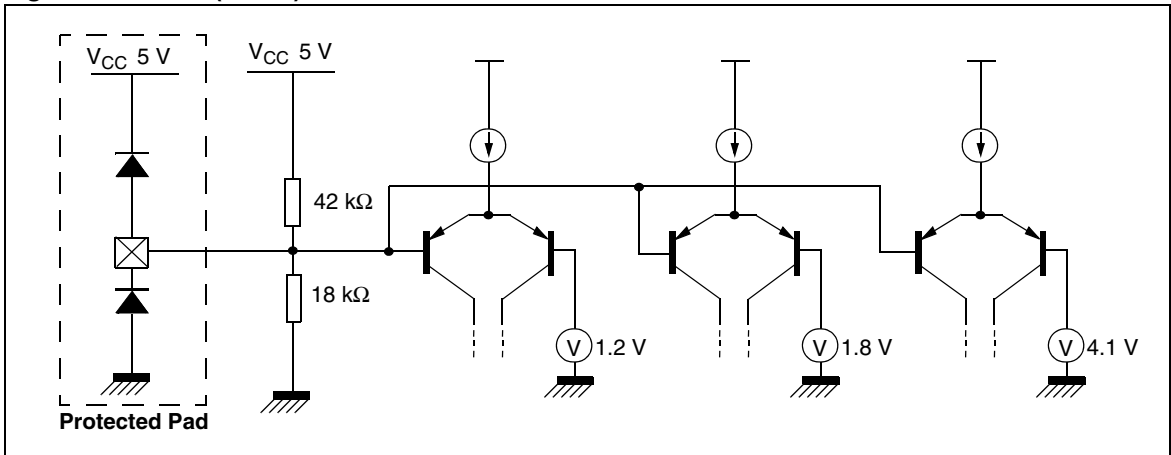
Figure 10. Mute (MUTE)
