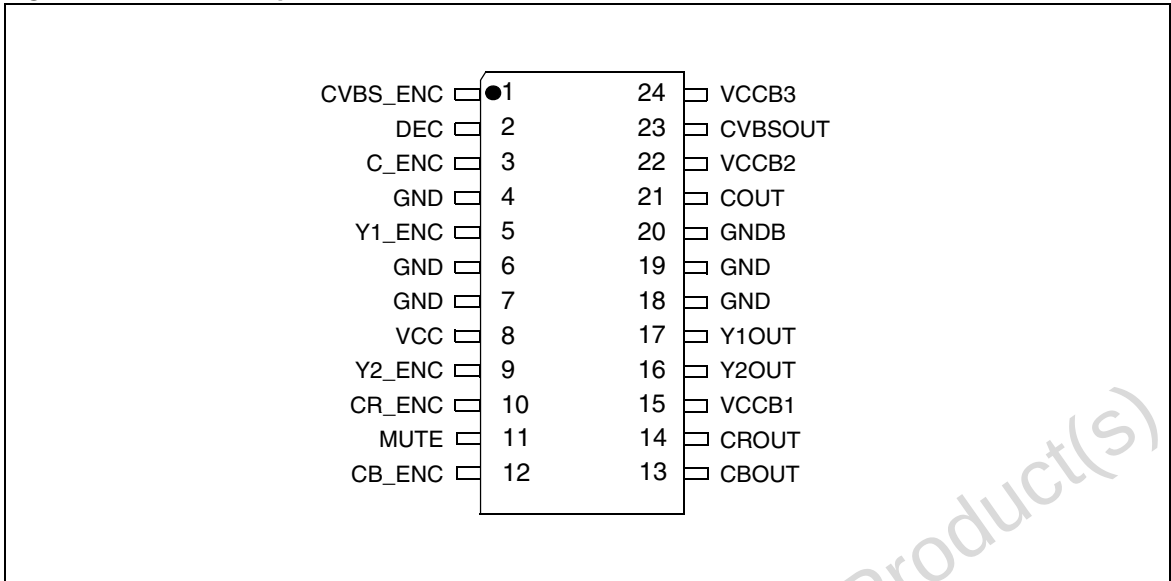
Figure 1. STV6436S pinout
