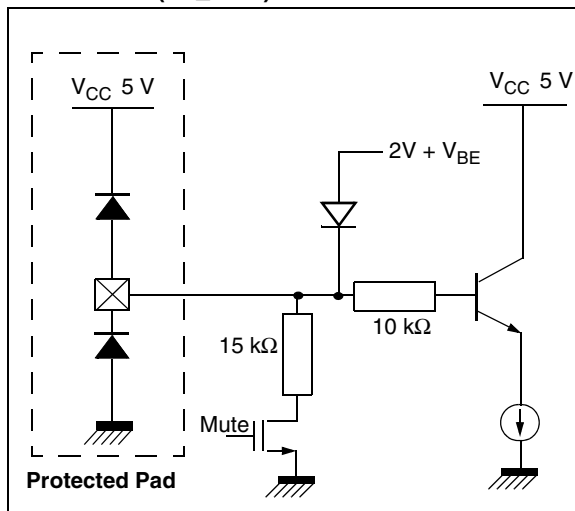
Figure 5. Video outputs (CVBSOUT, Y1OUT, Y2OUT, CROUT and CROUT)
