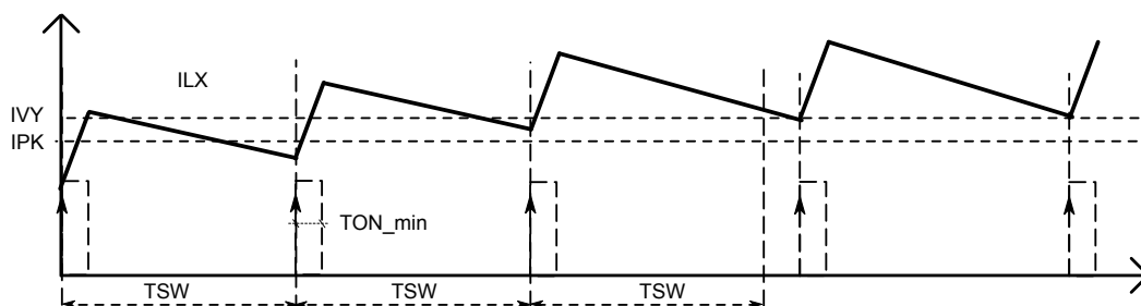
Figure 18. OCP – Valley current limit
