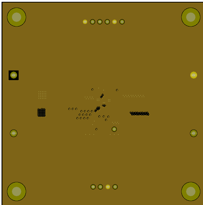
Figure 38. Evaluation board PCB layout. Internal layer 2.
