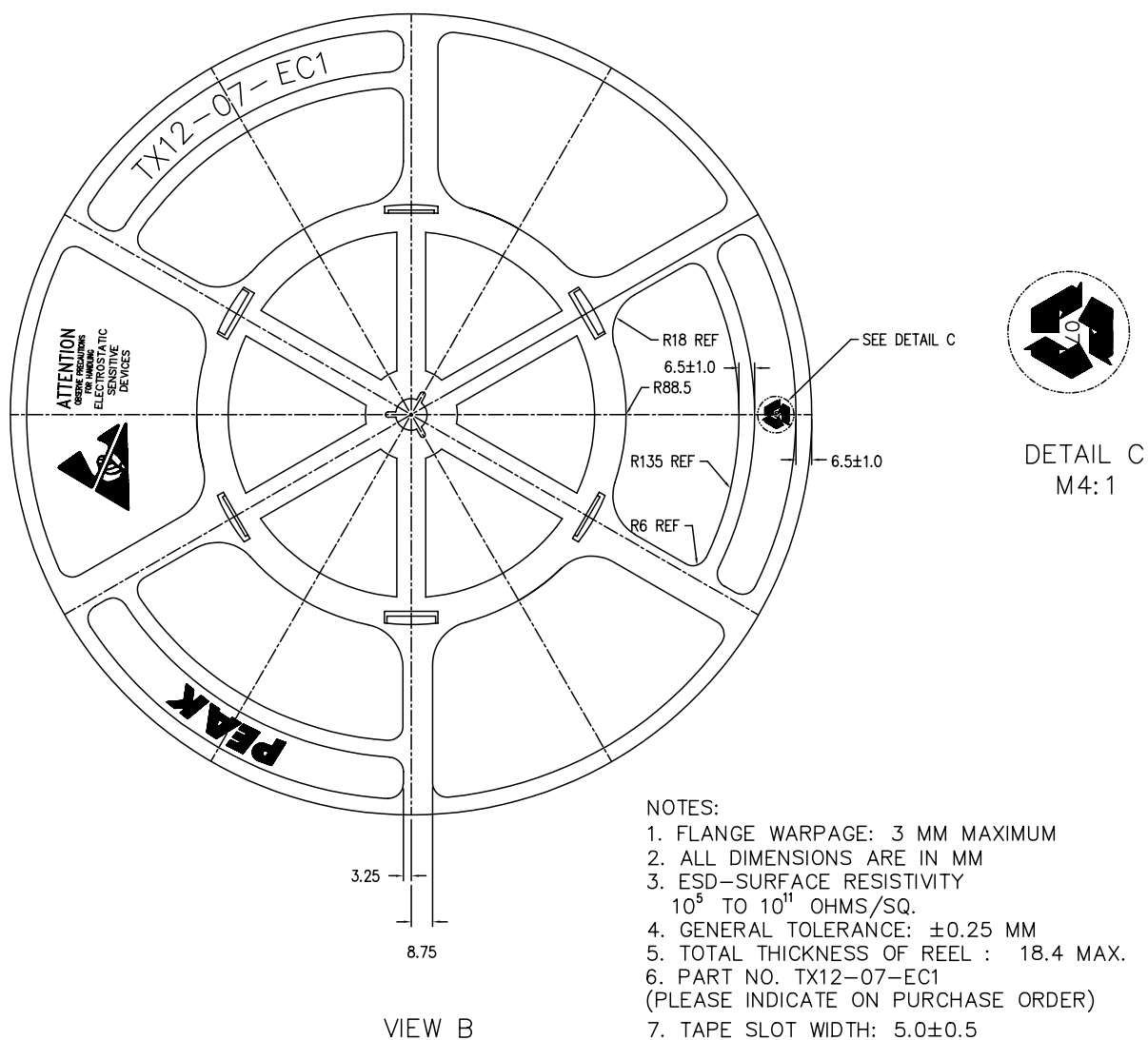
Figure 45. Reel drawing
