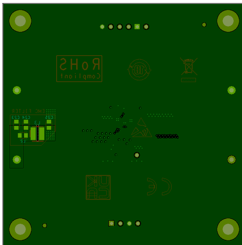
Figure 39. Evaluation board PCB layout. Bottom.
