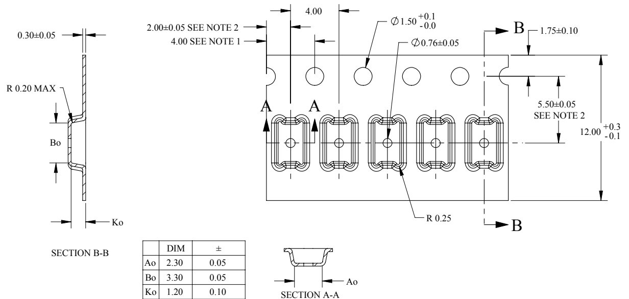
Figure 42. Carrier tape
