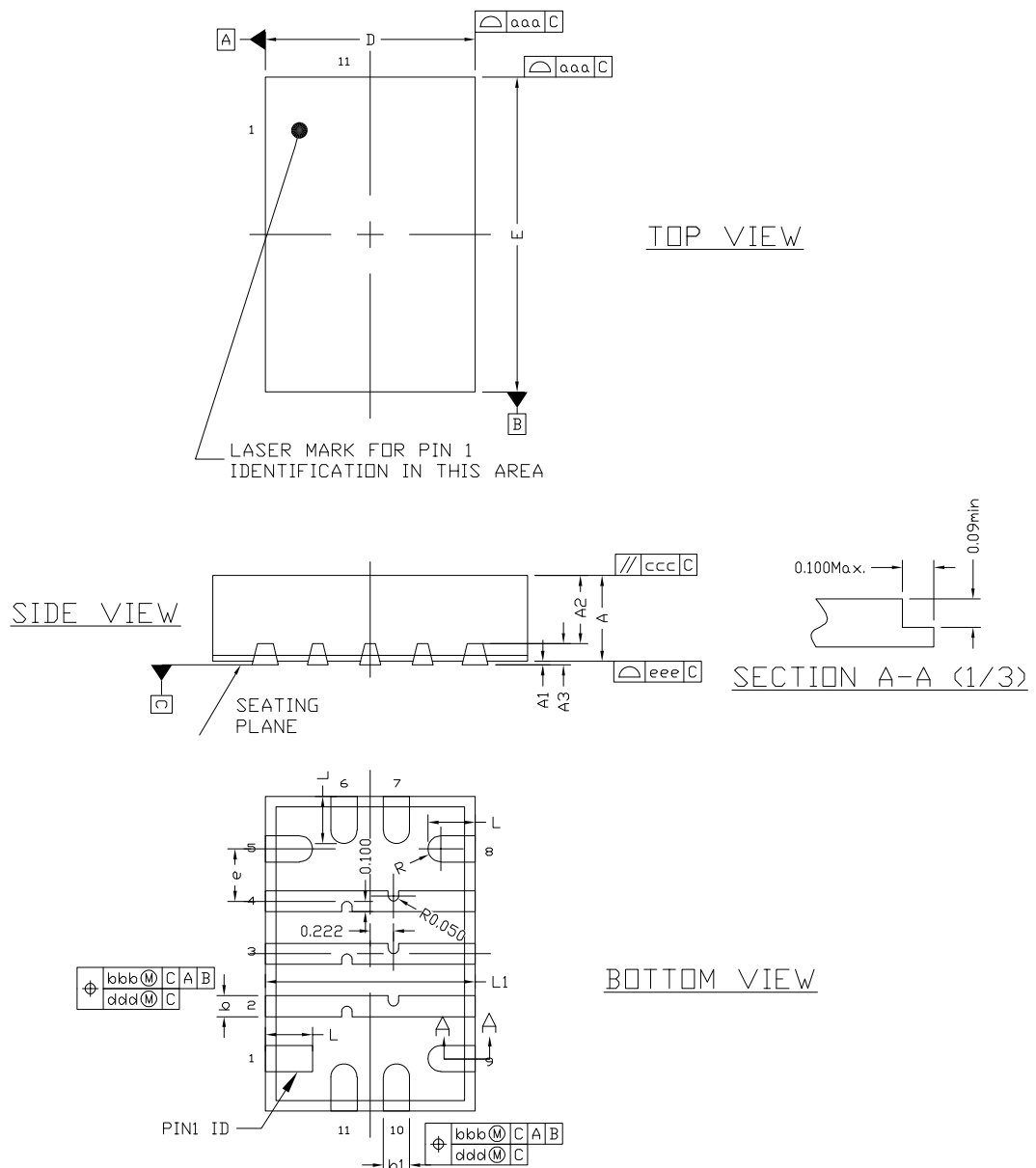
Figure 40. QFN11 (2 x 3 x 0.9 mm) package outline
