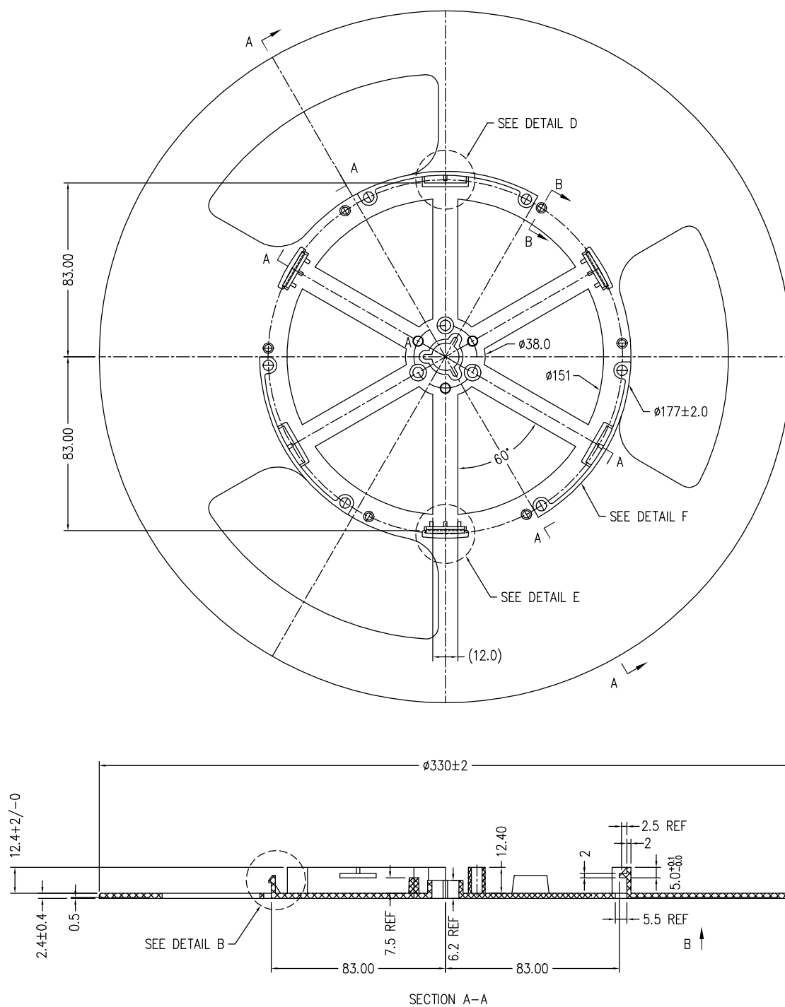
Figure 44. Carrier reel
