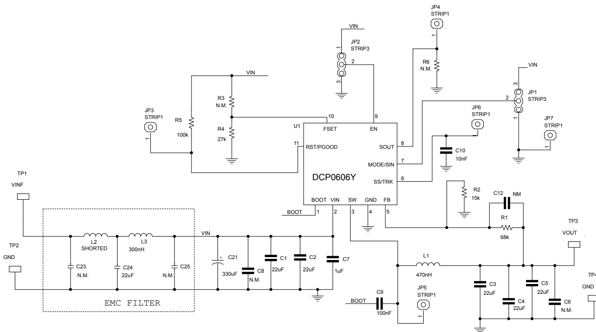
Figure 35. Evaluation board schematic
