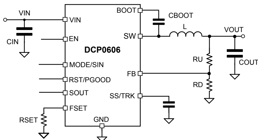
Figure 3. Typical application
