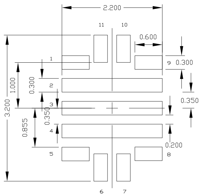
Figure 41. QFN11 (2 x 3 x 0.9 mm) recommended footprint - dimensions are in mm
