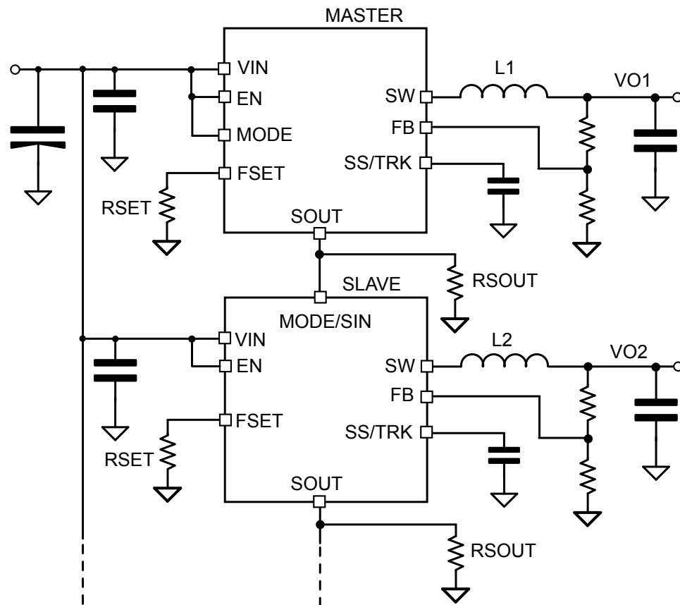
Figure 16. Synchronization example
