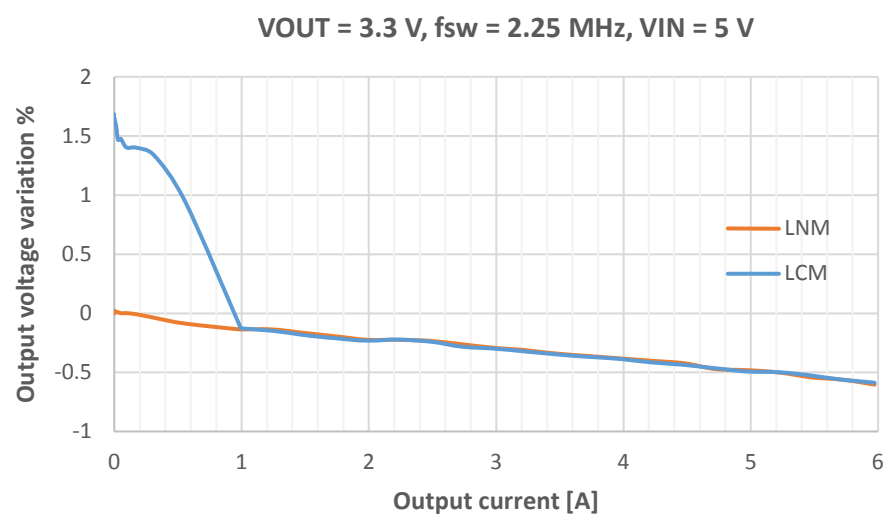
Figure 32. Load regulation
