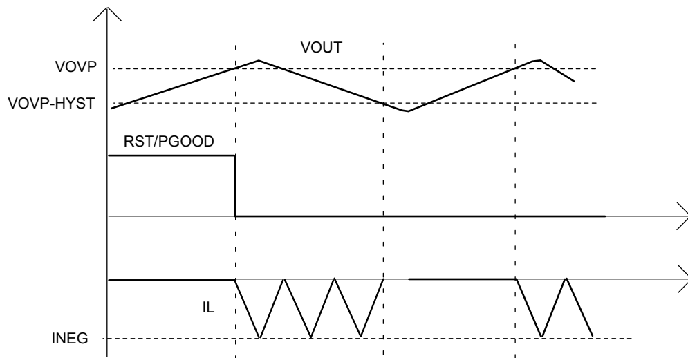
Figure 19. Output overvoltage protection
