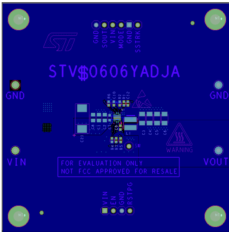
Figure 36. Evaluation board PCB layout. Top.
