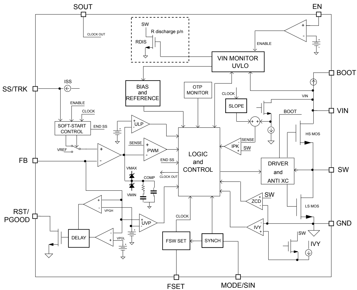
Figure 1. Block diagram
