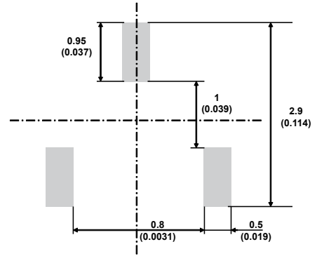
Figure 17. SOT23-3L footprint in mm (inches)
