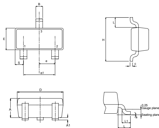
Figure 15. SOT23-3L package outline
