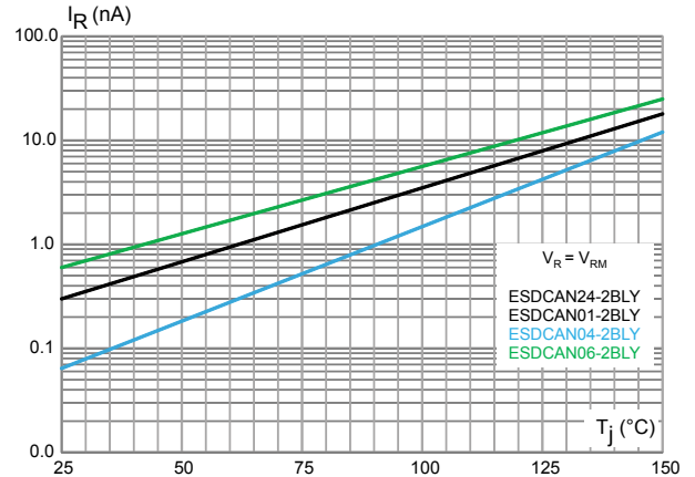
Figure 6. Leakage current versus junction temperature
