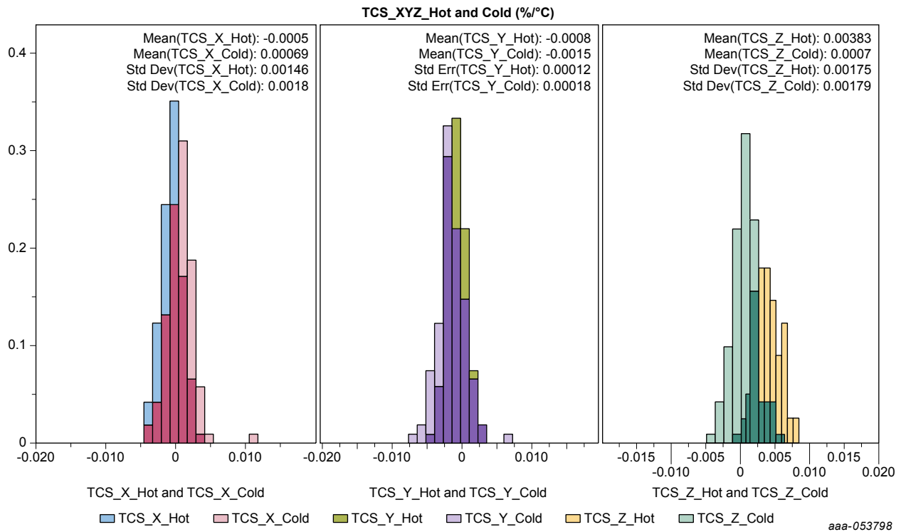
Figure 6. XYZ_TCS histograms
