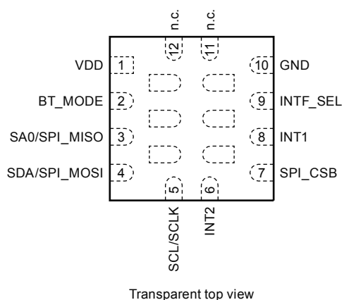
Figure 2. Pin configuration diagram
