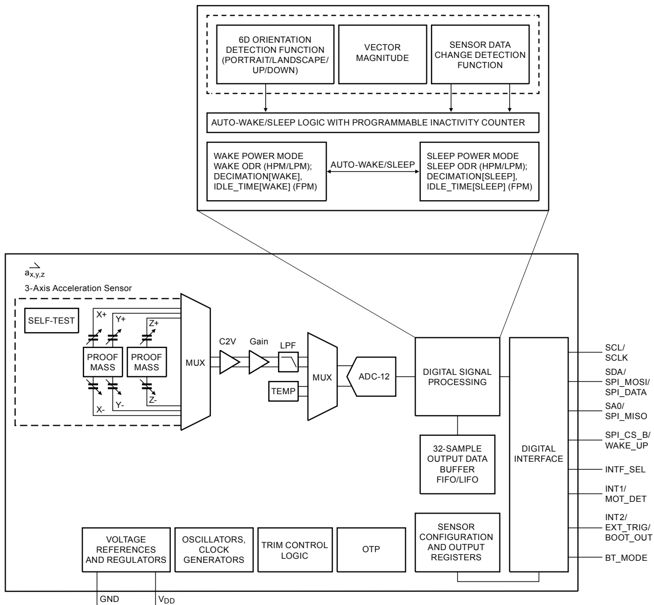
Figure 1. Block Diagram
