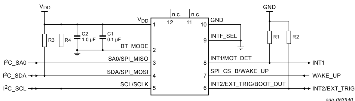
Figure 22. Typical Application Circuit #1 – I 2 C mode
