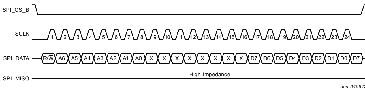
Figure 13. SPI single-byte read protocol diagram (3-wire mode)
