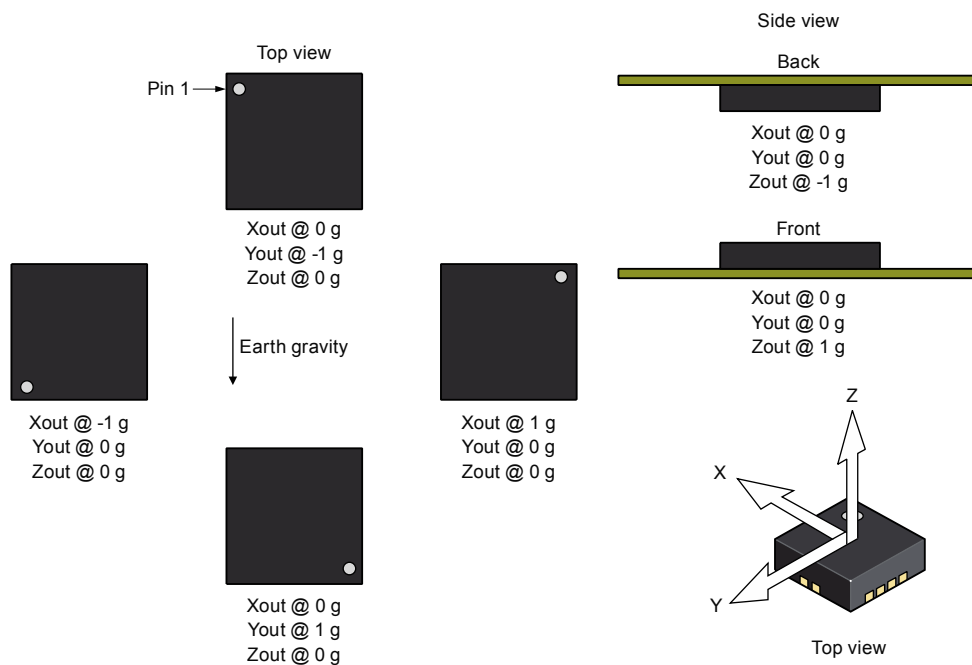
Figure 3. Sensitive axes orientation and output response to \pm 1 g (gravity) stimulus
