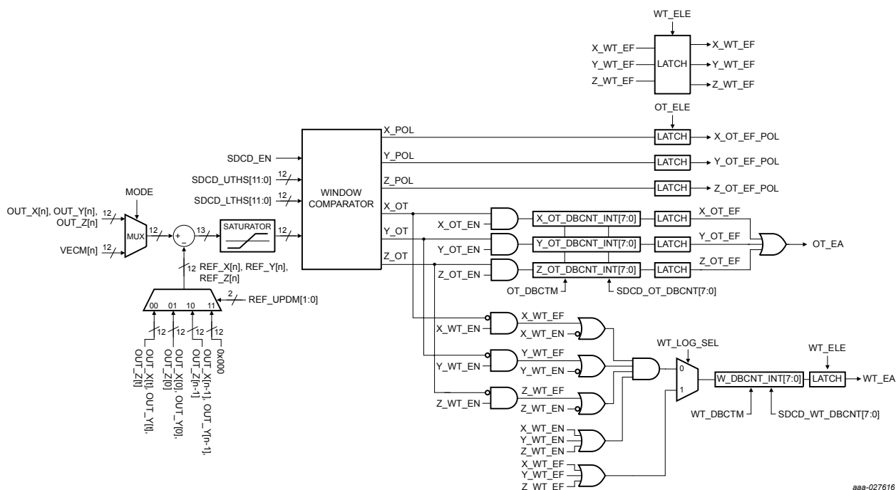
Figure 20. SDCD Function Block Diagram
