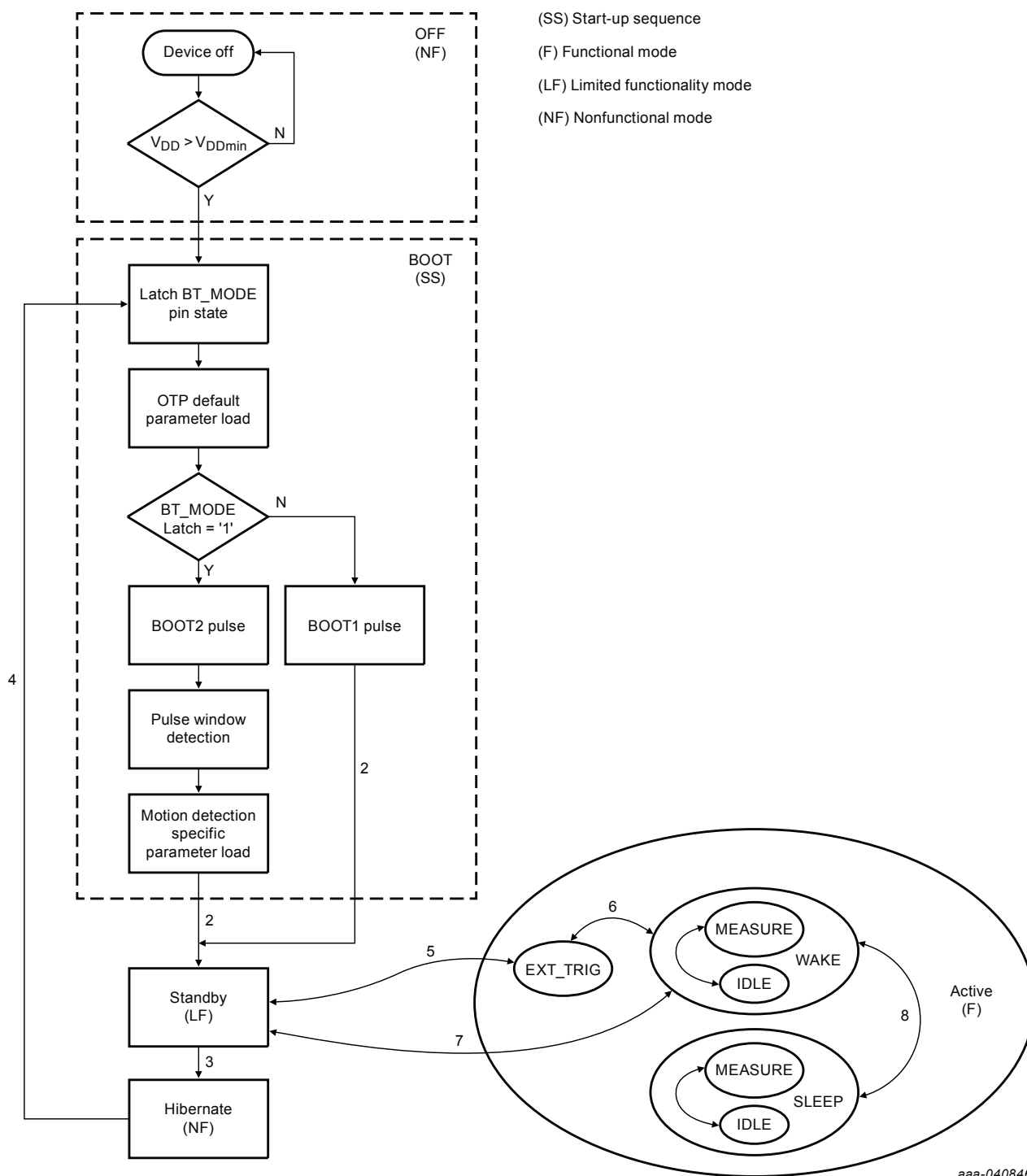
Figure 17. Operating modes transition diagram
