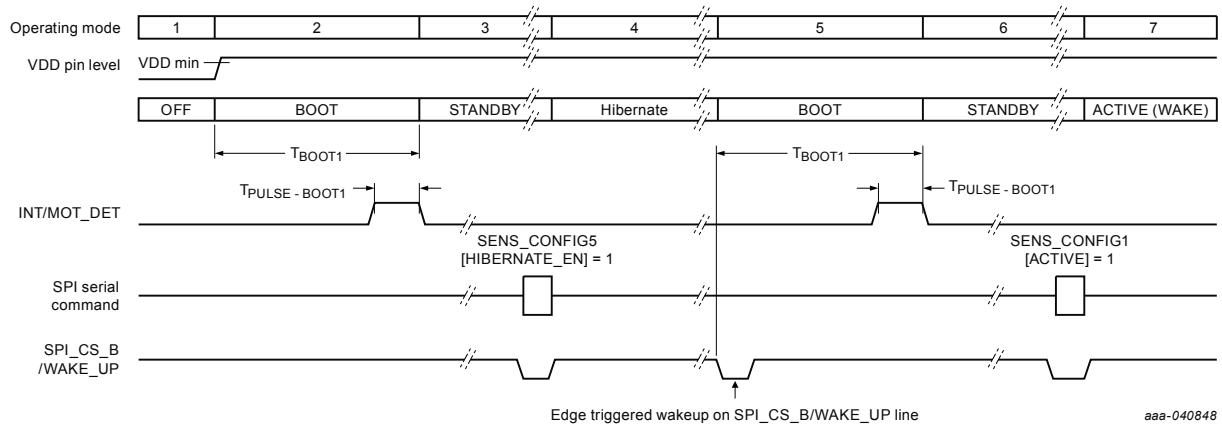
Figure 19. BOOT1 sequence (BT_MODE = GND)
