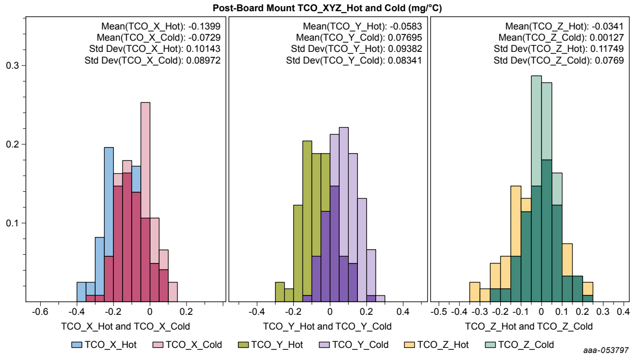
Figure 5. XYZ_TCO histograms
