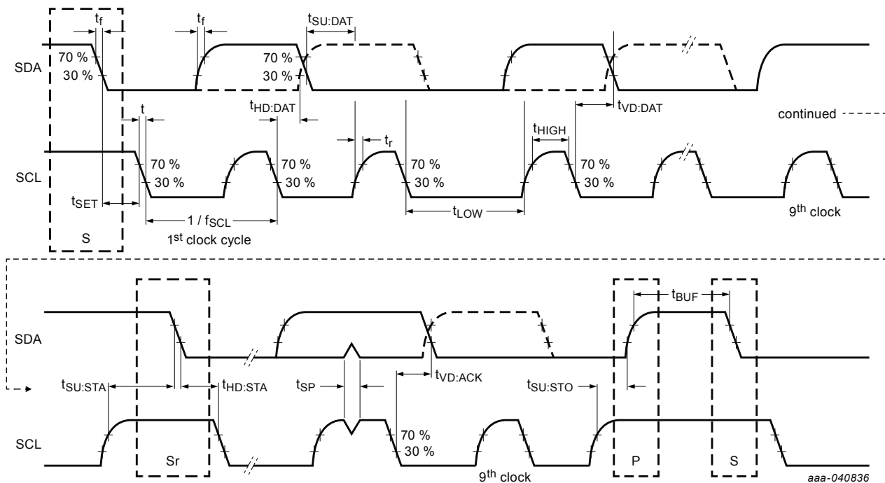
Figure 7. I 2 C secondary timing diagram for Standard-mode, Fast-mode and Fast-mode Plus
