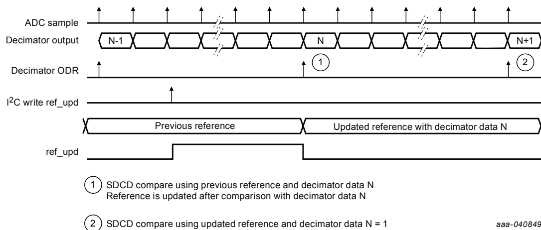
Figure 21. SDCD REF_UPD timing diagram
