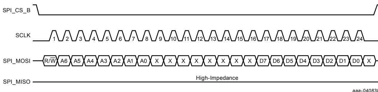
Figure 9. SPI single-byte write protocol diagram (3- or 4-wire mode), R/W = 0
