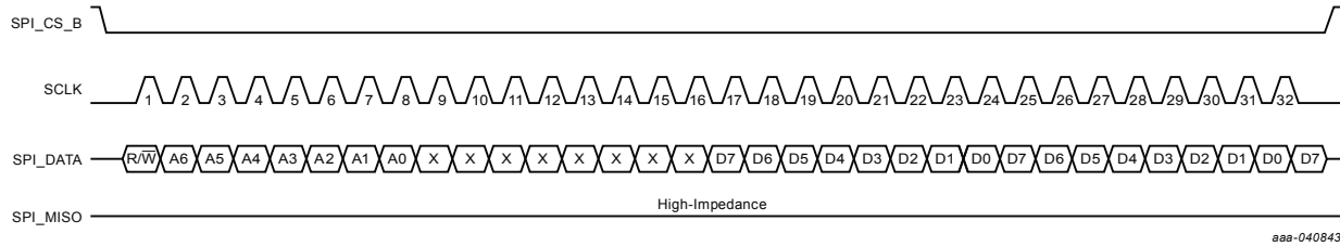
Figure 14. SPI multiple-byte read protocol diagram (3-wire mode)
