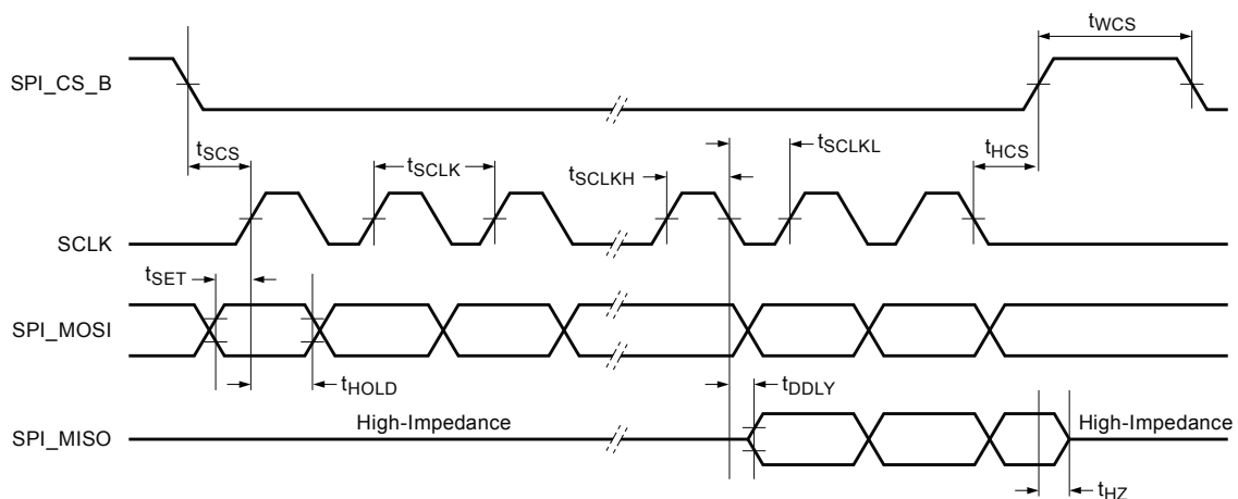
Figure 15. SPI timing diagram (4-wire mode)
