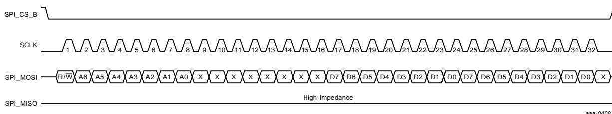
Figure 10. SPI multiple-byte write protocol diagram (3- or 4-wire mode), R/W = 0
