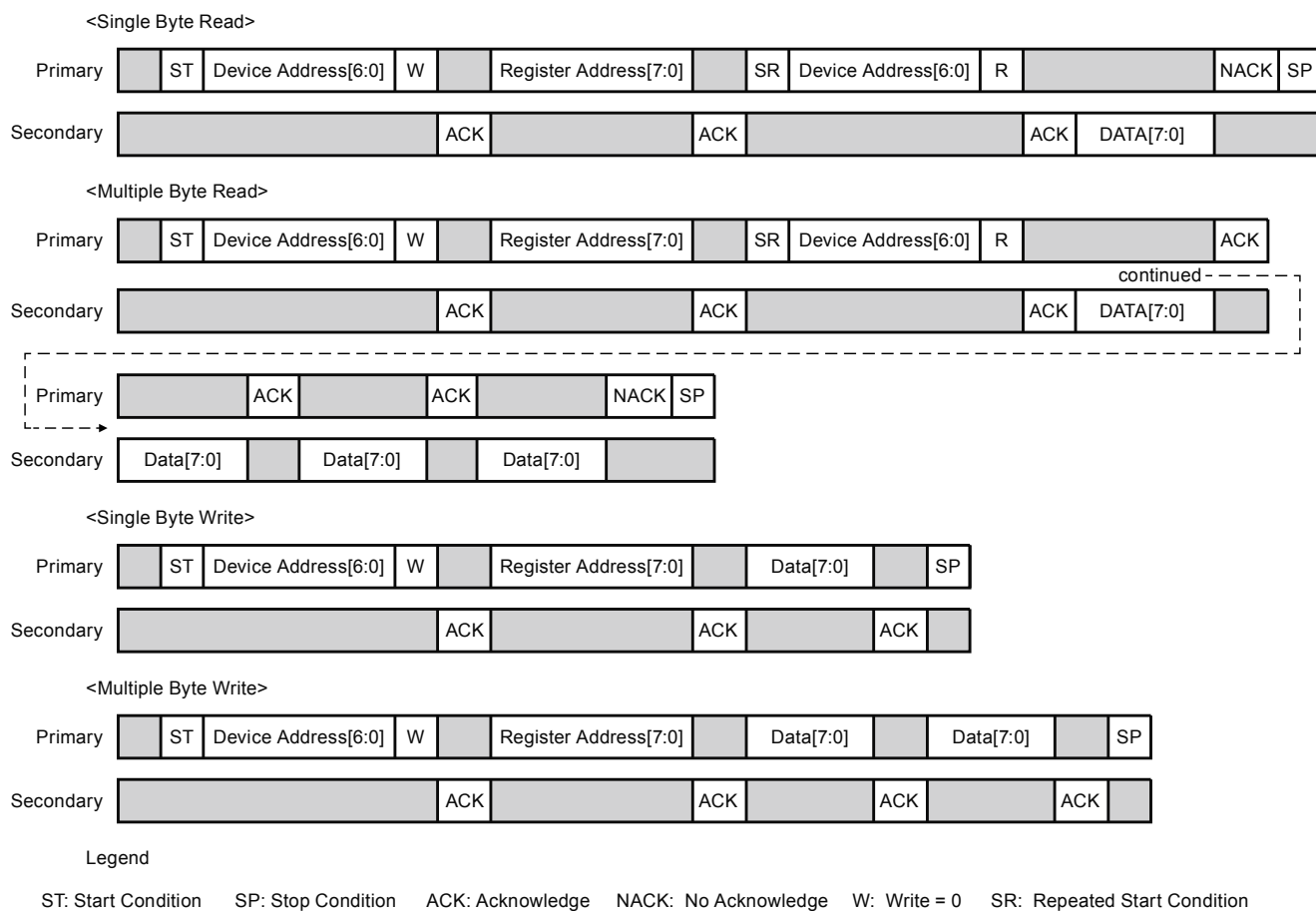
Figure 8. I 2 C Data Sequence Diagrams
