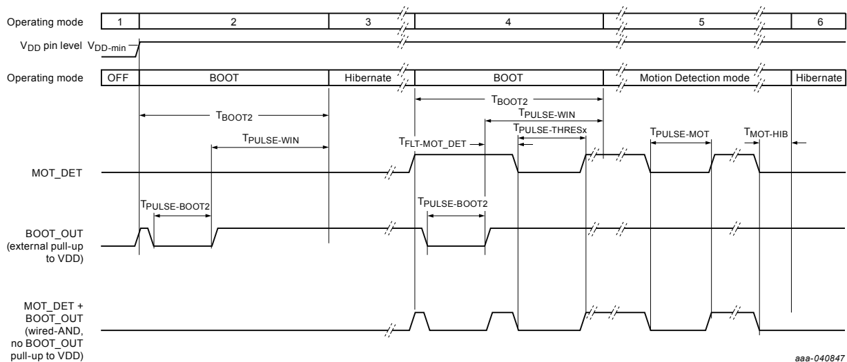
Figure 18. BOOT2 sequence and One-wire motion-detection protocol diagram (BT_MODE = V DD )
