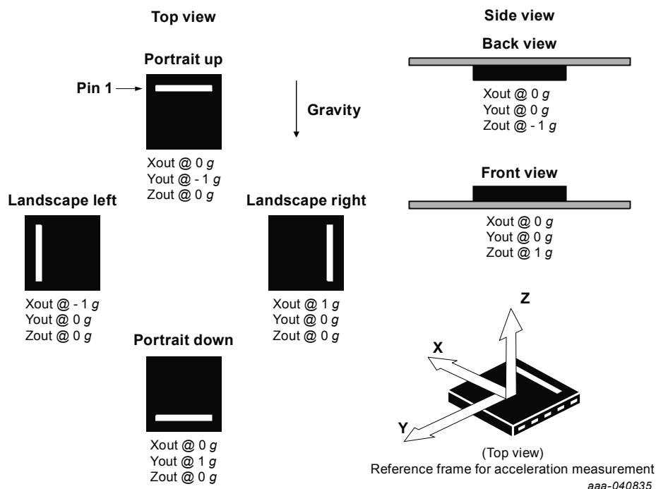
Figure 3. Sensitive axes orientation and output response to ±1 g (gravity) stimulus
