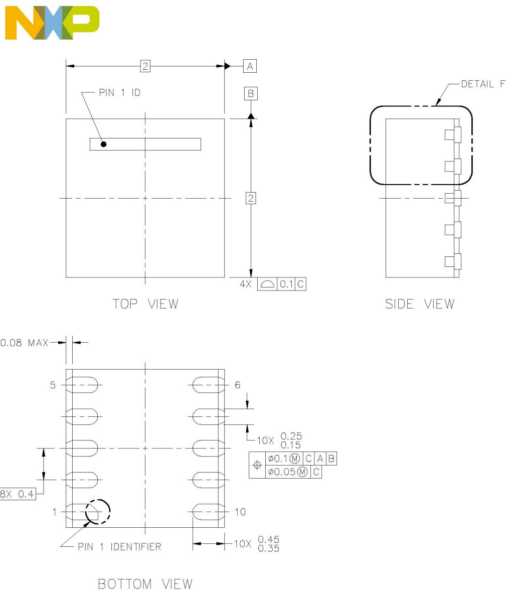
Figure 25. FXLS8964AF package outline
