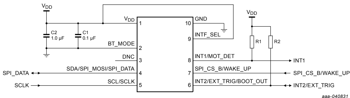
Figure 21. Typical Application Circuit #3 – SPI 3-wire mode (software enabled; SENS_CONFIG1[SPI_M] = 1)
