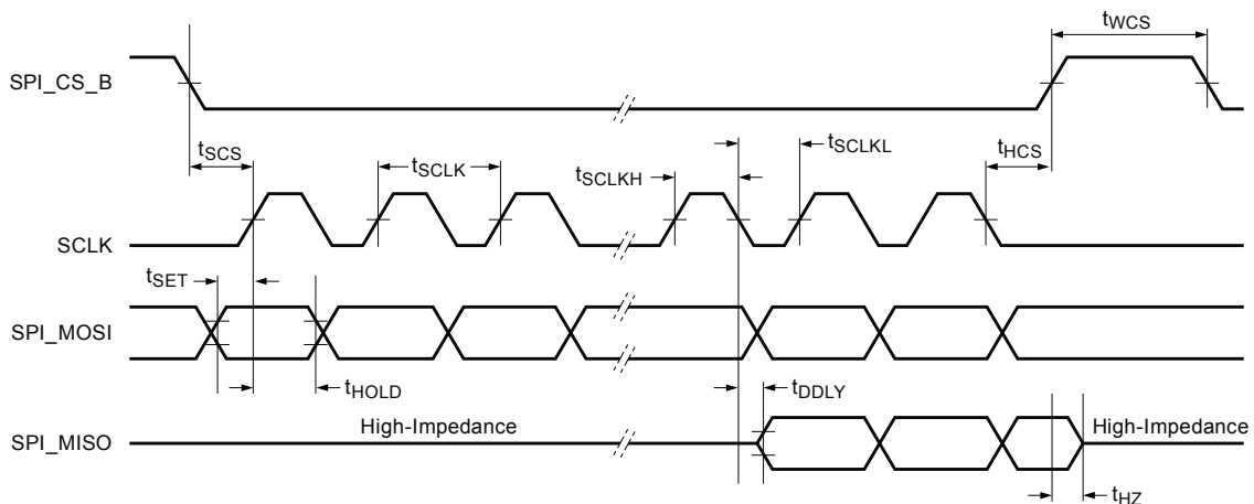
Figure 12. SPI timing diagram (4-wire mode)
