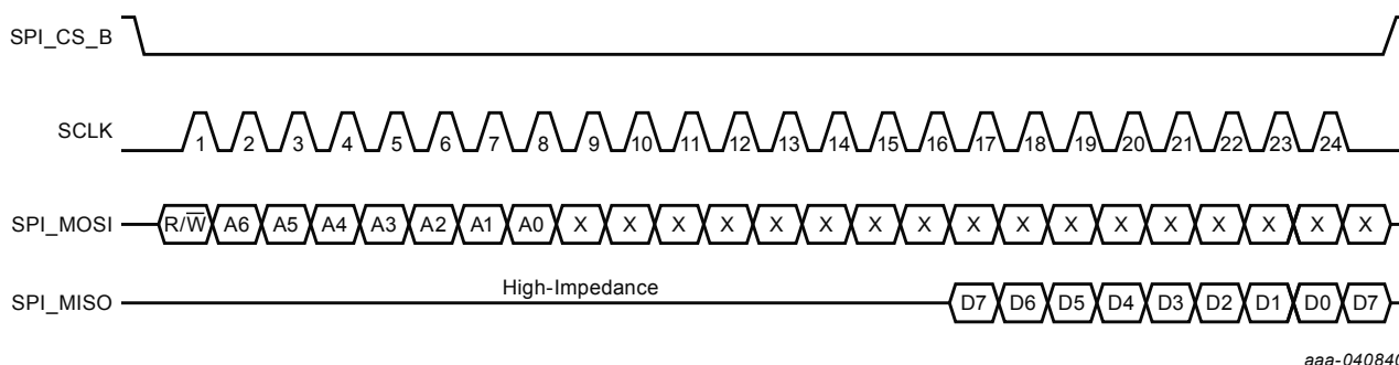
Figure 8. SPI single-byte read protocol diagram (4-wire mode), R/W = 1
