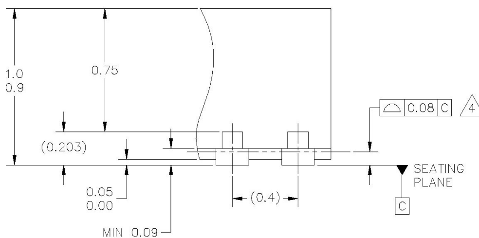
DETAIL F VIEW ROTATED 90°CW
