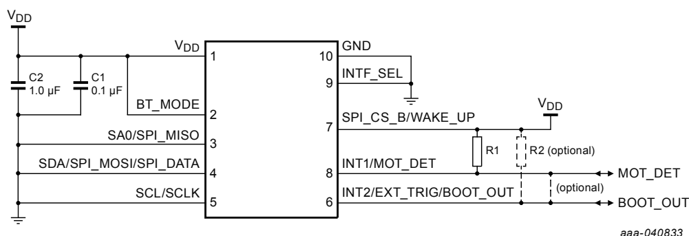
Figure 23. Typical Application Circuit #5 – Motion detection mode (no serial interface)
