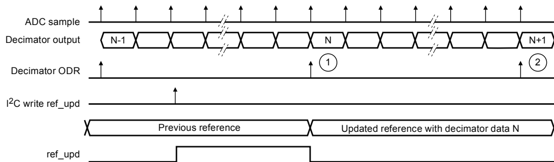
Figure 18. SDCD REF_UPD timing diagram
