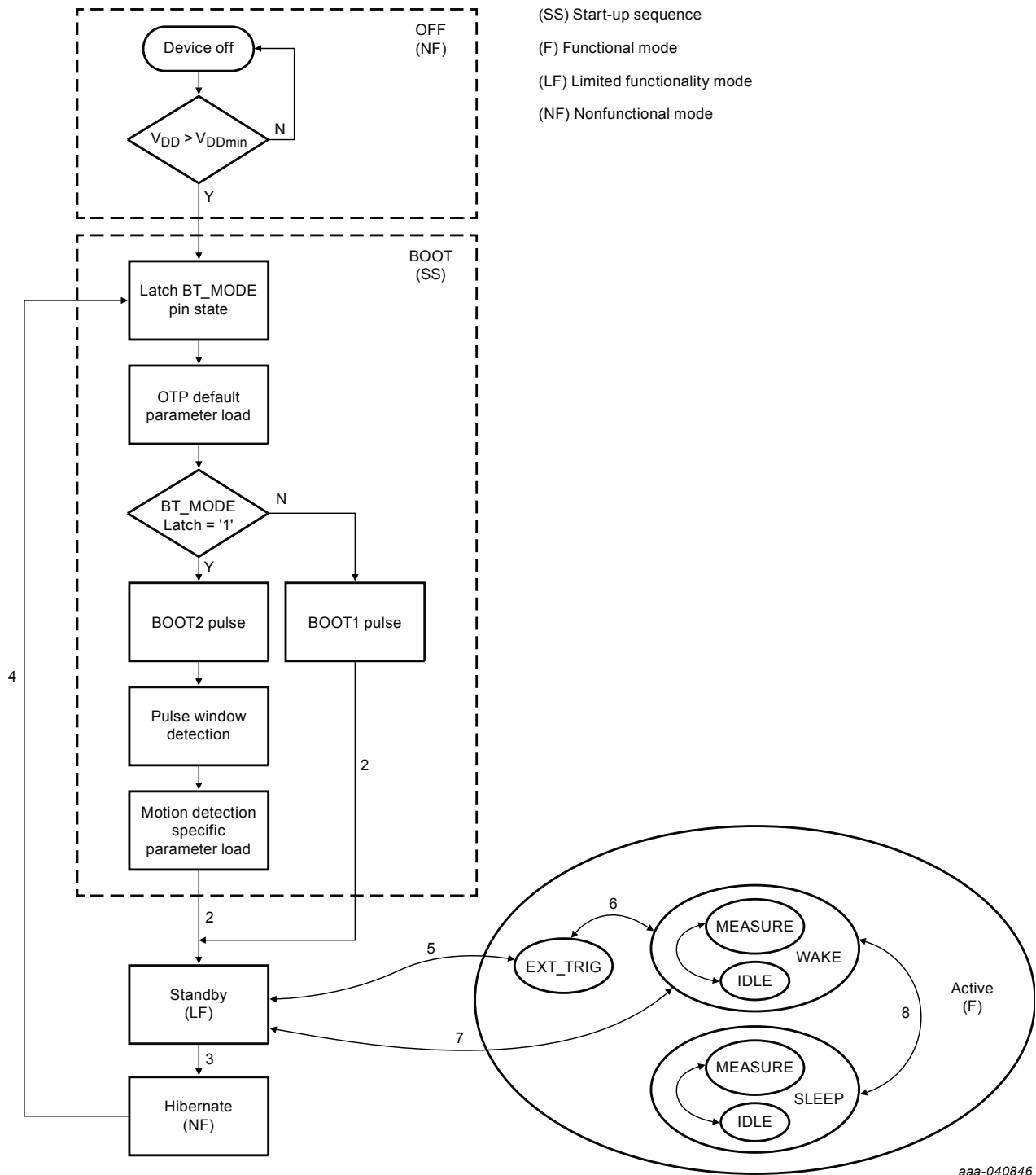
Figure 14. Operating modes transition diagram
