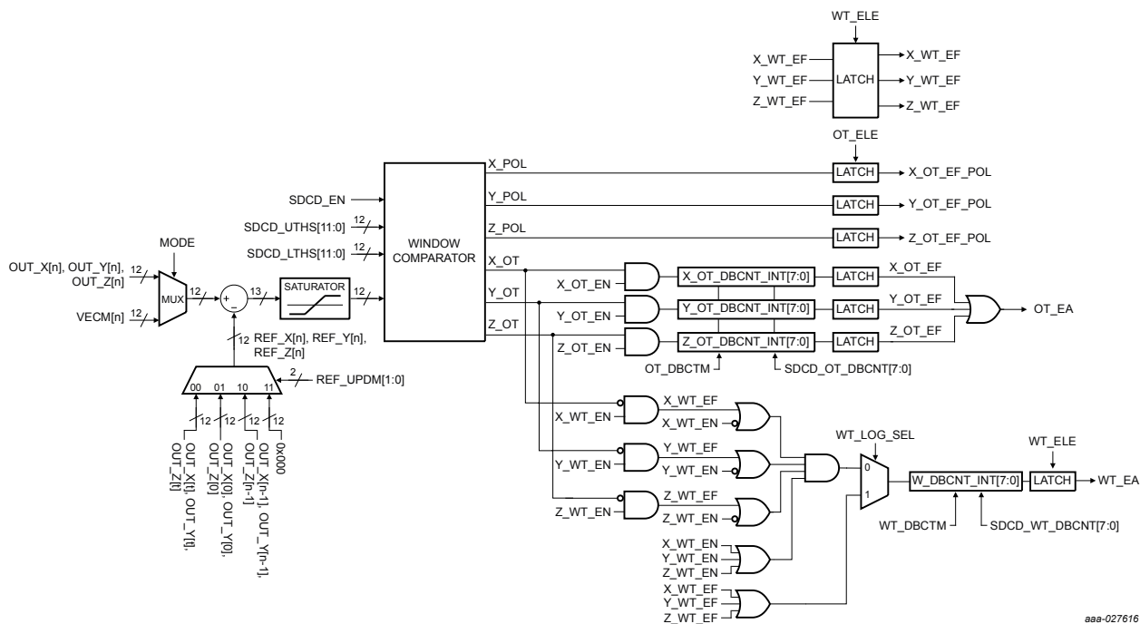
Figure 17. SDCD Function Block Diagram
