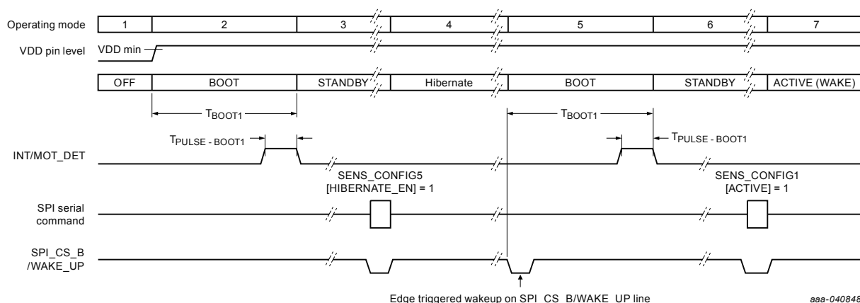
Figure 16. BOOT1 sequence (BT_MODE = GND)
