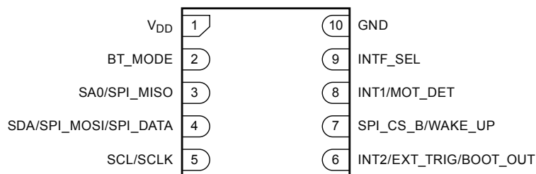
Figure 2. Pin configuration diagram
