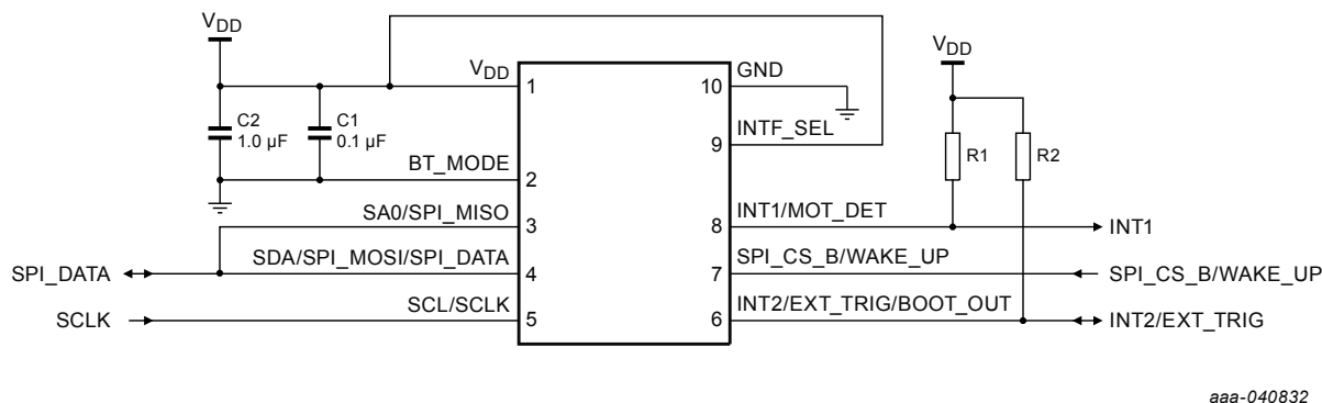
Figure 22. Typical Application Circuit #4 – SPI 3-wire mode (hardwired; SENS_CONFIG1[SPI_M] = X)
