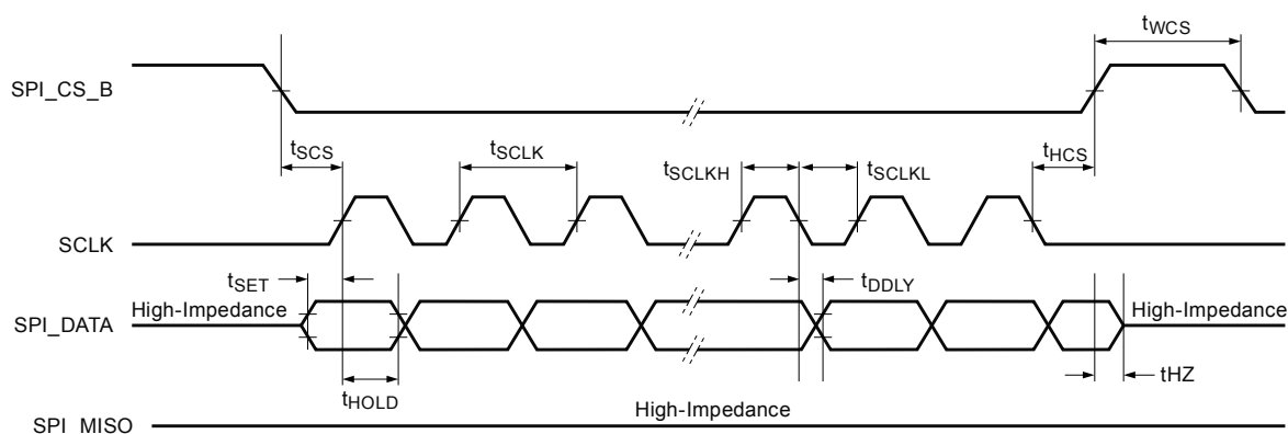
Figure 13. SPI timing diagram (3-wire mode)
