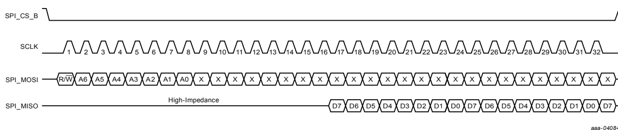
Figure 9. SPI multiple-byte read protocol diagram (4-wire mode), R/W = 1
