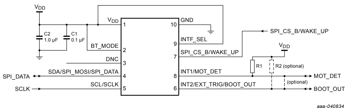
Figure 24. Typical Application Circuit #6 - Motion detection mode (with SPI 3-wire interface, software enabled)
