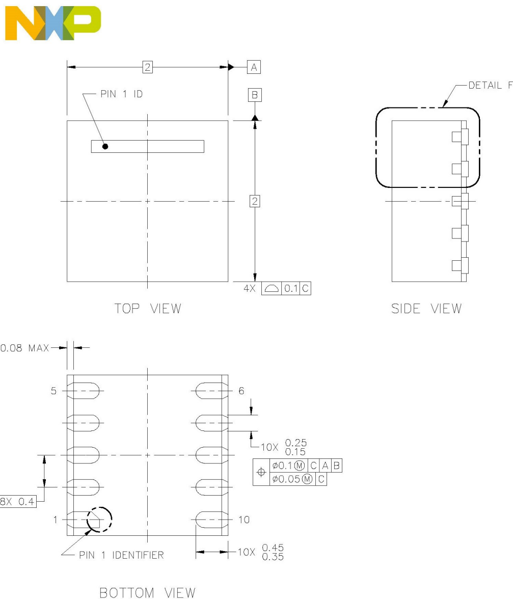
Figure 25. FXLS8967AF package outline
