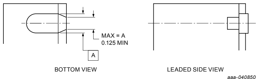
Figure 28. Bottom and leaded view dimensions
