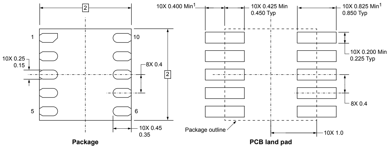
Figure 29. PCB footprint guidelines
