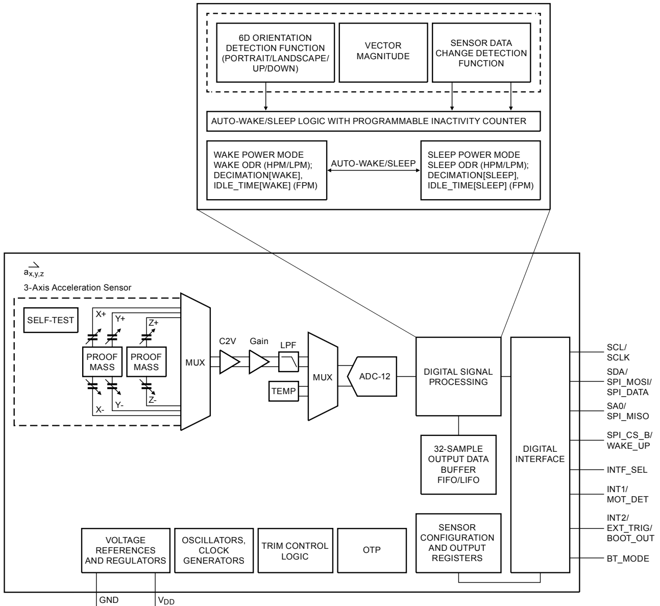
Figure 1. Block Diagram
