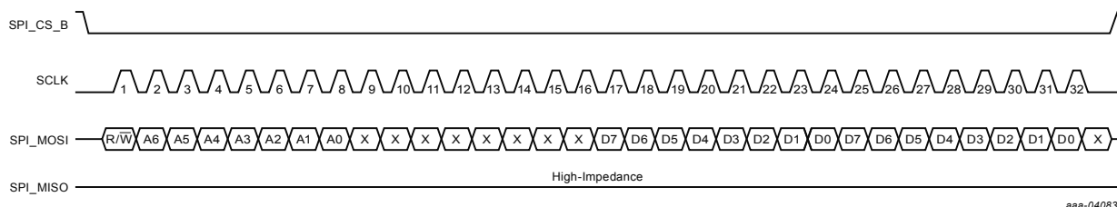
Figure 7. SPI multiple-byte write protocol diagram (3- or 4-wire mode), R/W = 0
