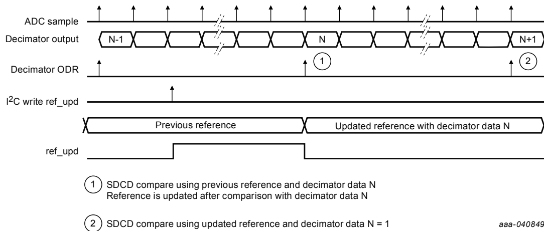
Figure 18. SDCD REF_UPD timing diagram
