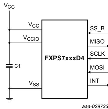
Figure 26. SPI application diagram for FXPS7115Dx4S
