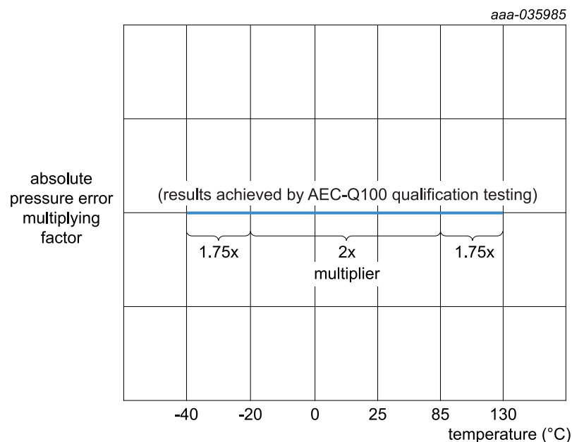
Figure 24. Absolute pressure accuracy multiplier over life
