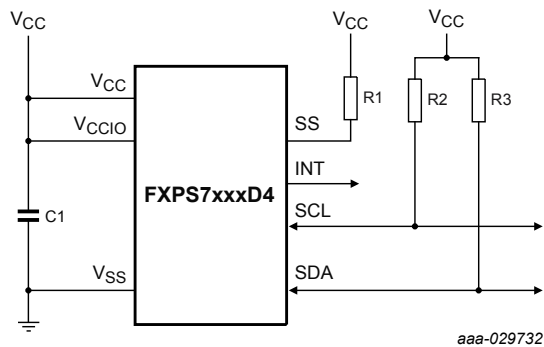
Figure 25. I 2 C application diagram of FXPS7115Dx4S
