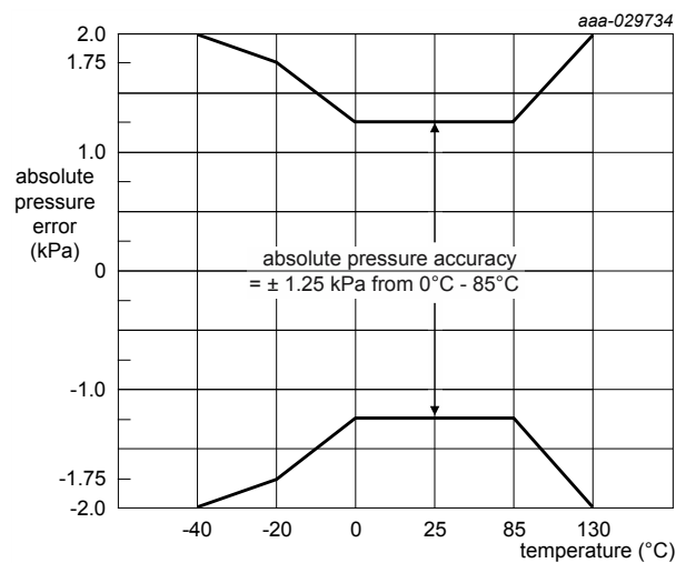
Figure 23. Absolute pressure accuracy as a function of temperature
