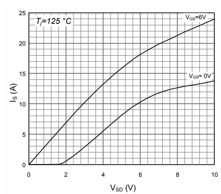
Figure 8. Typ I_S vs. V_{SD} at T_J = 125^\circ\text{C}
