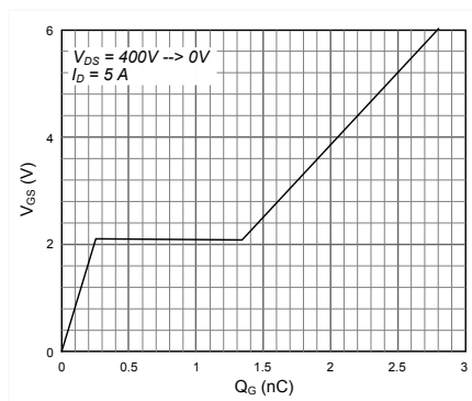
Figure 11. Typ Gate charge at T_J = 25\text{ °C}
