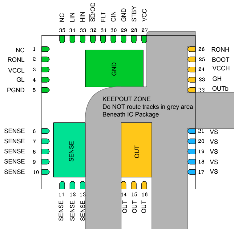
Figure 16. Keepout regions for safety
