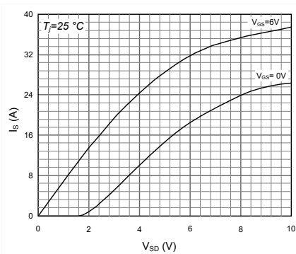
Figure 7. Typ I_S vs. V_{SD} at T_J = 25^\circ\text{C}
