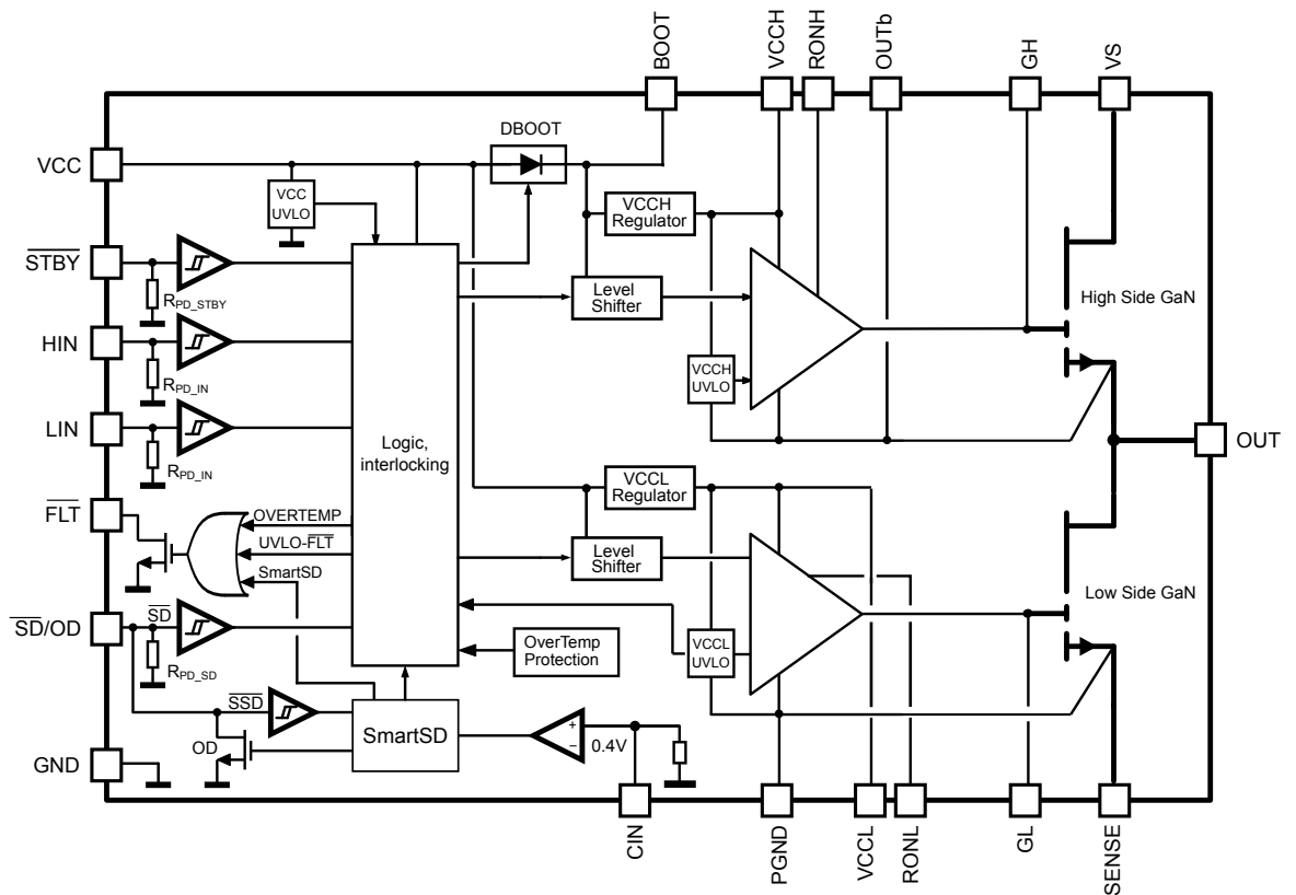
Figure 1. GANSPIN611 block diagram
