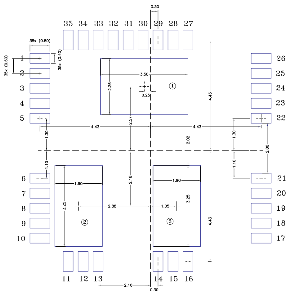
Figure 18. QFN 9 x 9 x 1 mm, 35 leads, 0.6 mm pitch, suggested footprint
