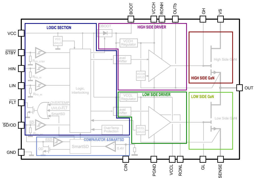
Figure 13. GANSPIN611 simplified block diagram
