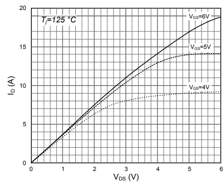
Figure 6. Typ I_D vs. V_{DS} at T_J = 125^\circ\text{C}
