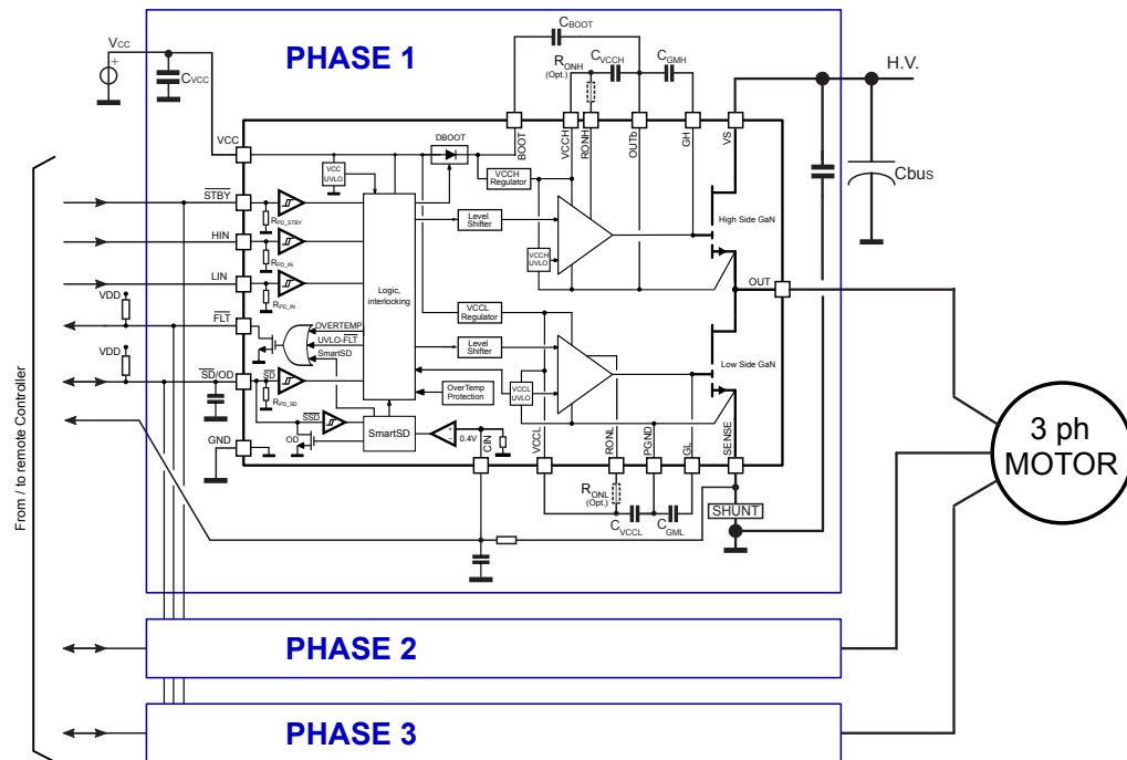
Figure 2. Typical motor control application schematic
