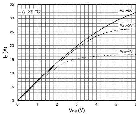
Figure 5. Typ I_D vs. V_{DS} at T_J = 25^\circ\text{C}
