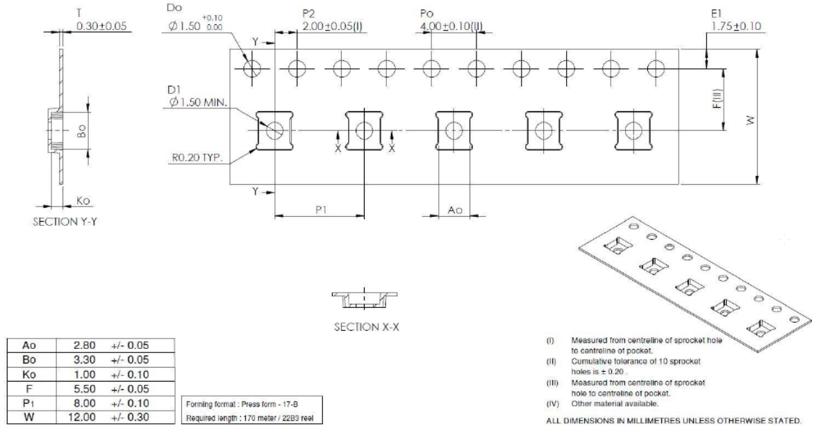
Figure 24. LGA-14L package orientation in carrier tape
