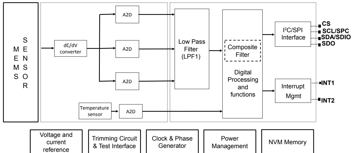
Figure 9. Accelerometer architecture
