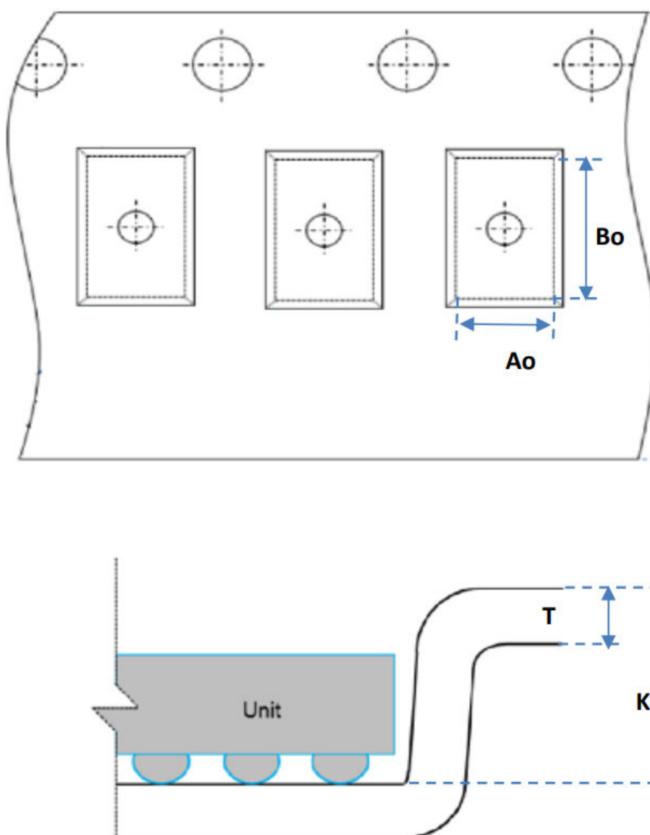
Figure 23. VFQFPN-48L reel shipment reference
