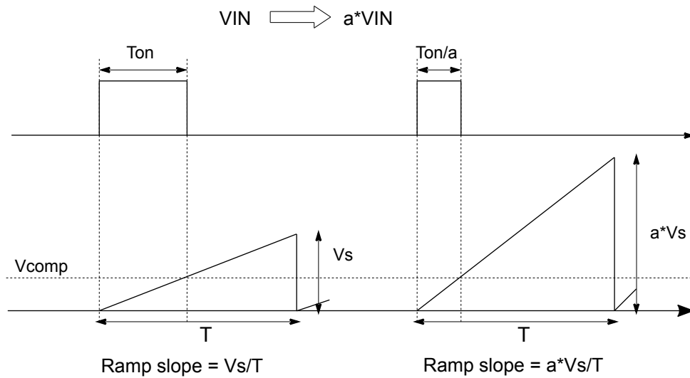
Figure 7. Internal sawtooth ramp feedforward - Fsw adjusted by external resistor
