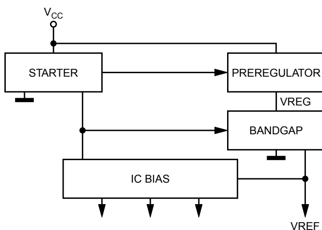
Figure 6. Internal circuit
