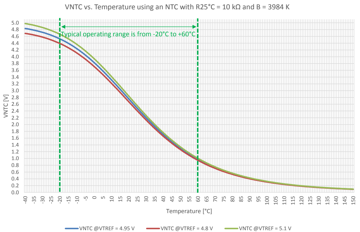
Figure 44. VNTC vs. temperature example (single ended measurement)
