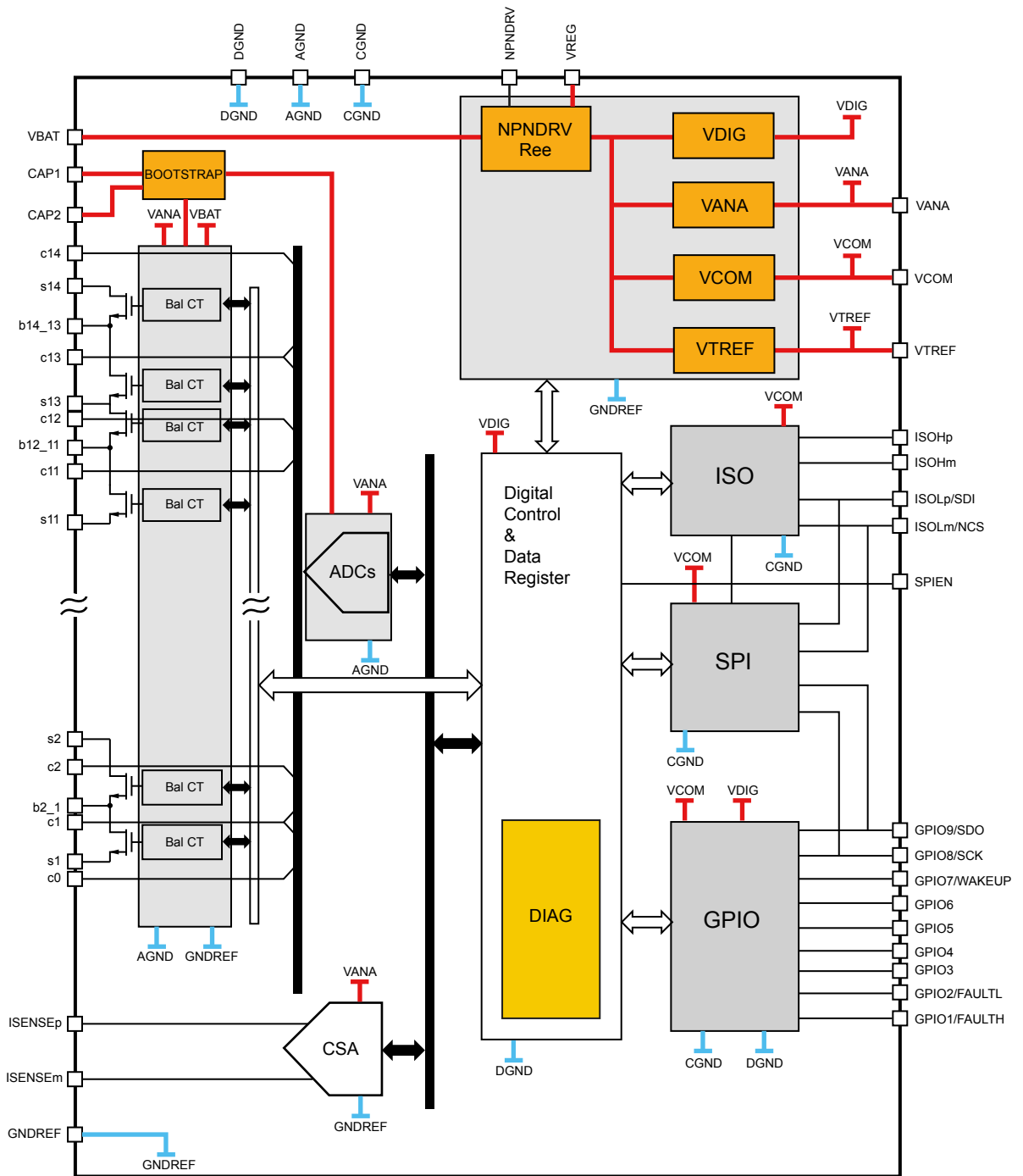
Figure 2. Block diagram
