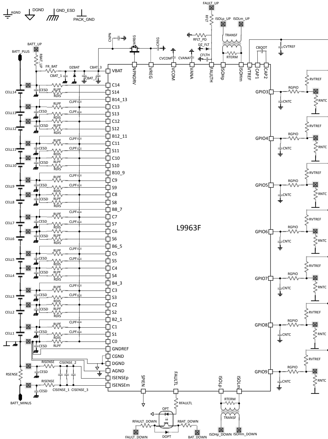
Figure 1. Typical application
