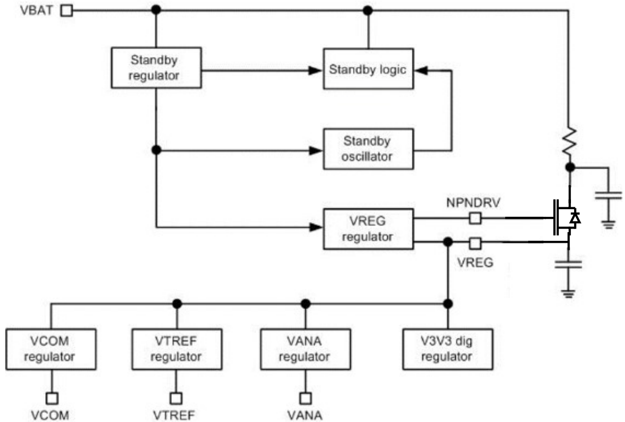
Figure 18. Regular scheme
