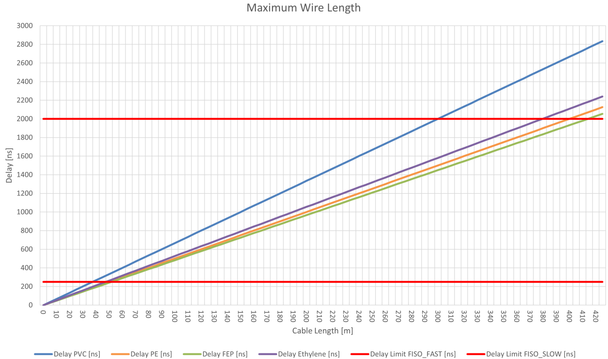
Figure 54. Maximum wire length according to wire insulator and operating frequency
