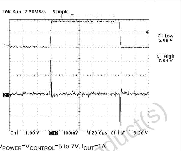
Figure 15. Line transient response V_{\text{Power}}=5\text{ V}
