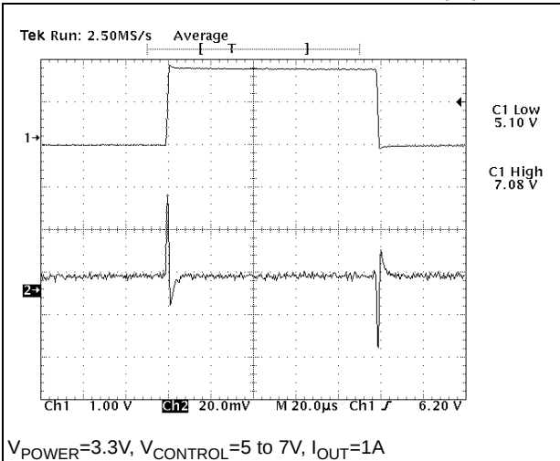
Figure 14. Line transient response V_{\text{Power}}=3.3\text{ V}
