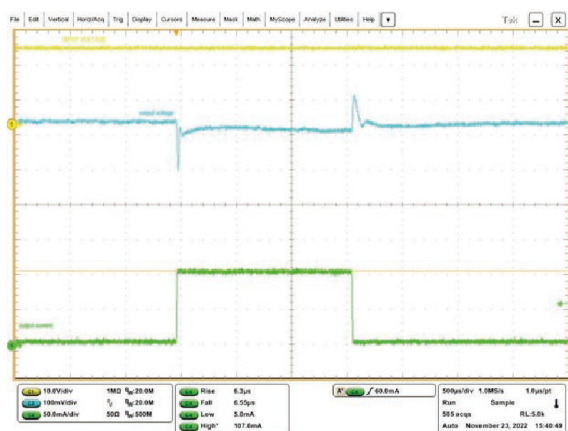
Figure 17. Load transient
